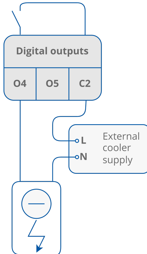
Figure 7. Electrical cooler connection
