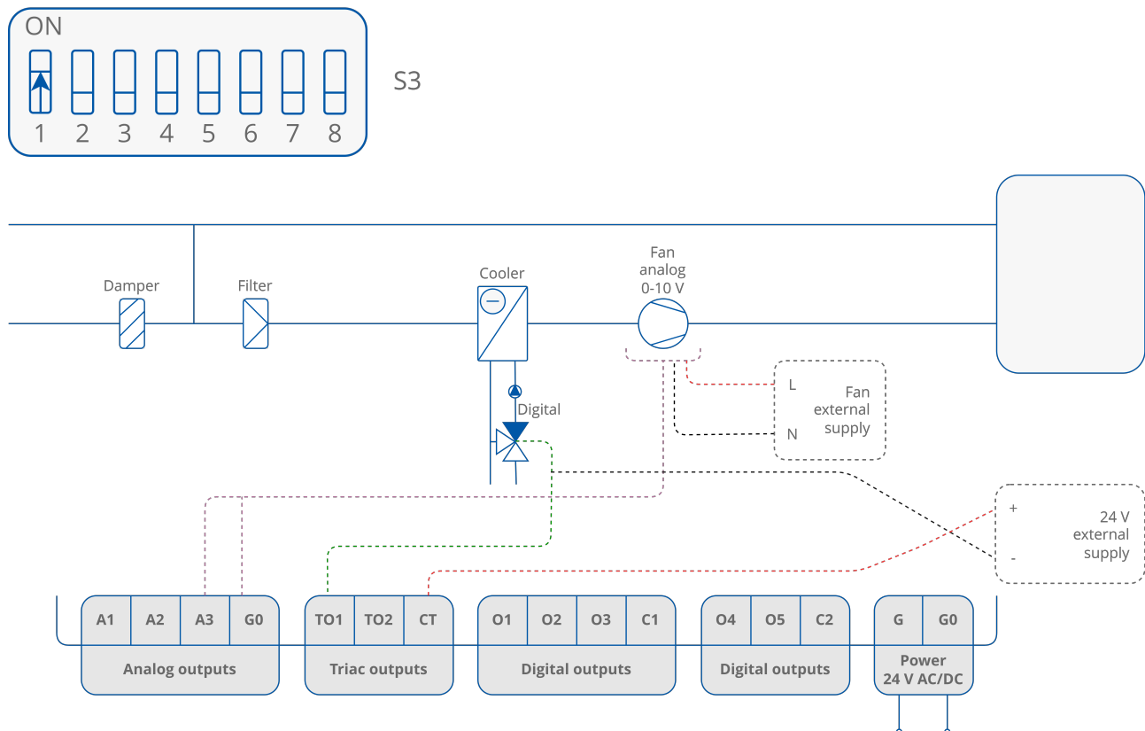
Figure 49. 2-pipe installation with 1-stage digital controlled cooling and analog controlled fan
