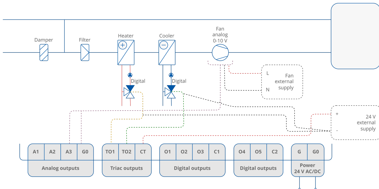
Figure 37. 4-pipe installation with 1-stage digital controlled heating and cooling and analog controlled fan
