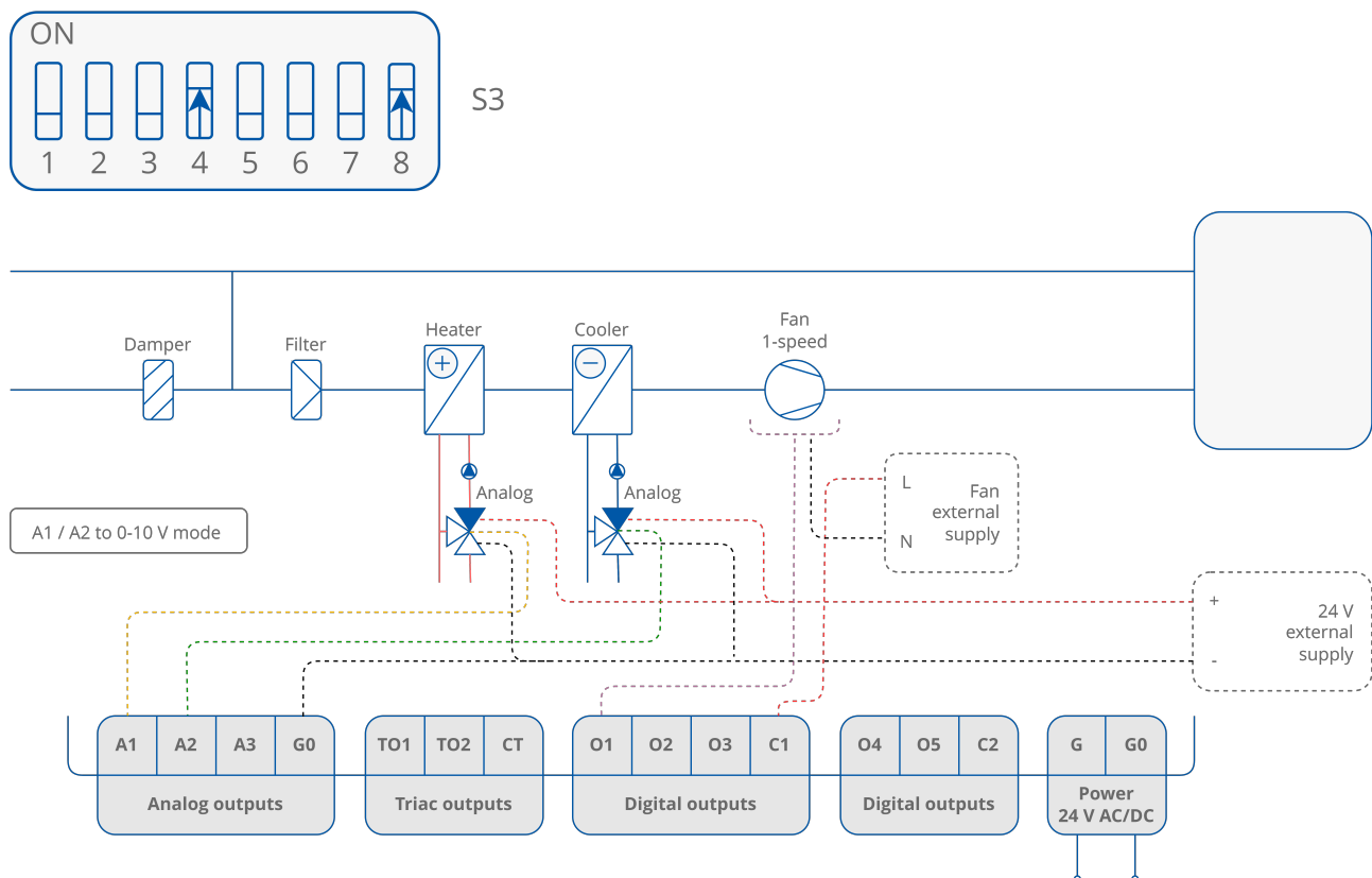
Figure 43. 4-pipe installation with 1-stage analog controlled heating and cooling and 1-speed fan - valve in analog mode
