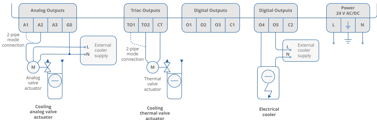
Figure 18. Cooling actuators connection
