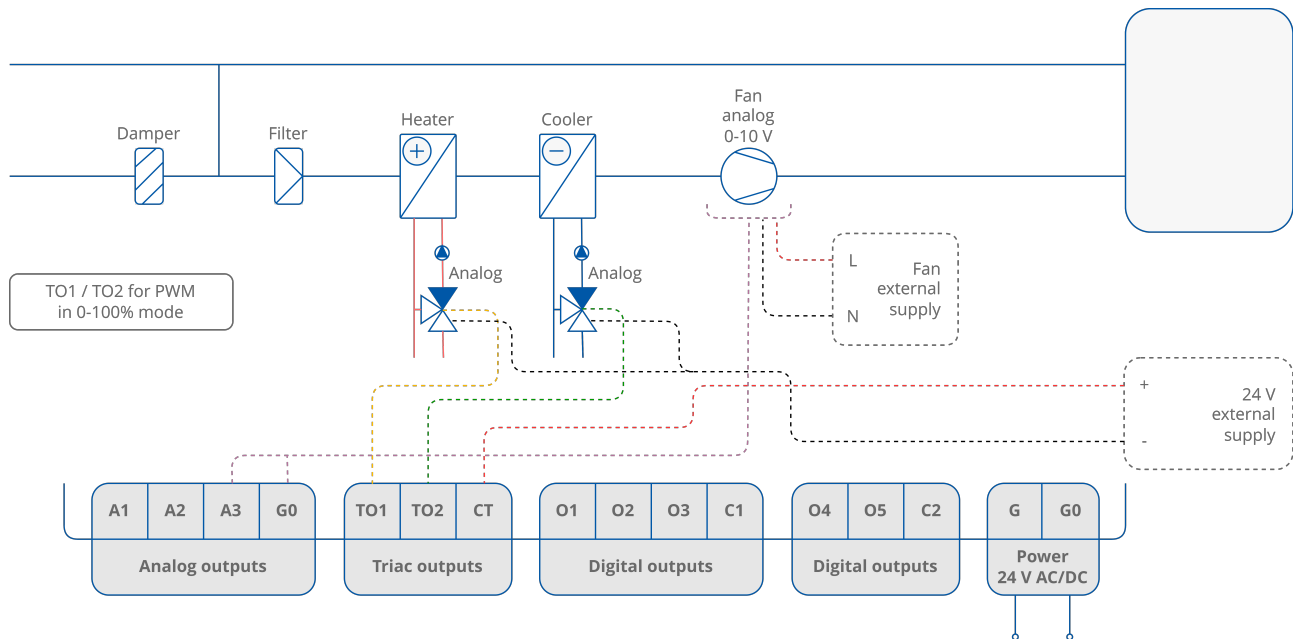
Figure 42. 4-pipe installation with 1-stage analog controlled heating and cooling and analog controlled fan - valve in PWM mode
