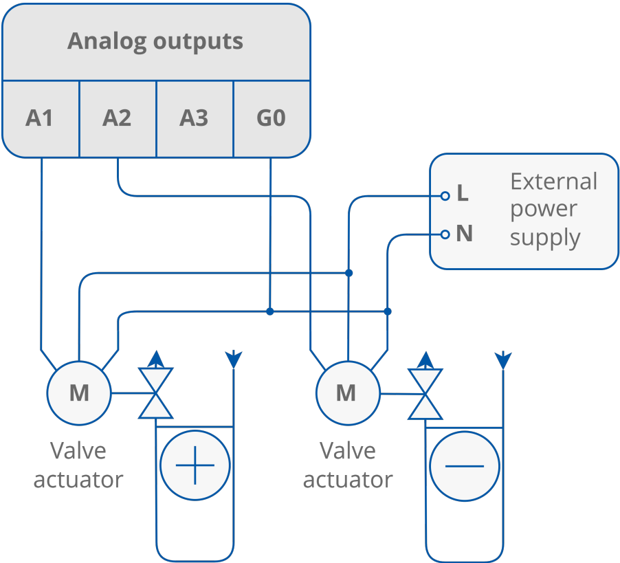
Figure 8. Connection of analog valve actuators
