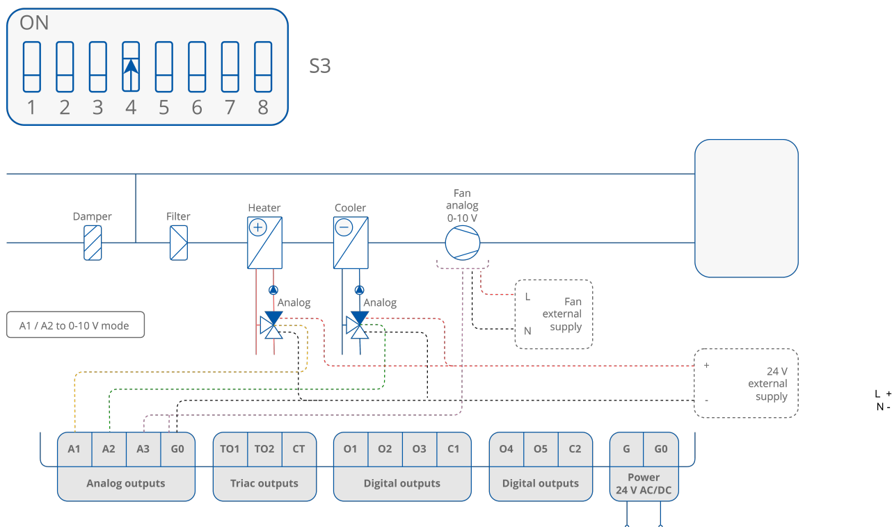
Figure 41. 4-pipe installation with 1-stage analog controlled heating and cooling and analog controlled fan - valve in analog mode
