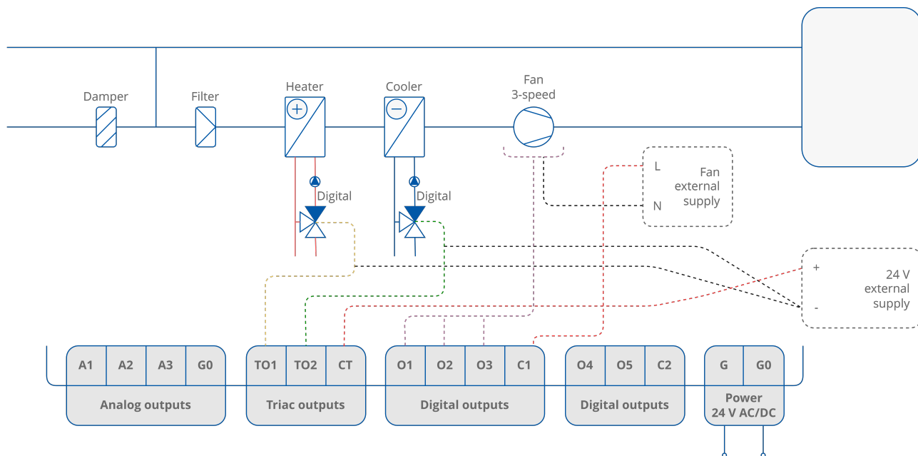
Figure 40. 4-pipe installation with 1-stage digital controlled heating and cooling and 3-speed fan
