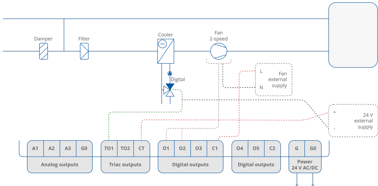
Figure 51. 2-pipe installation with 1-stage digital controlled cooling and 2-speed fan
