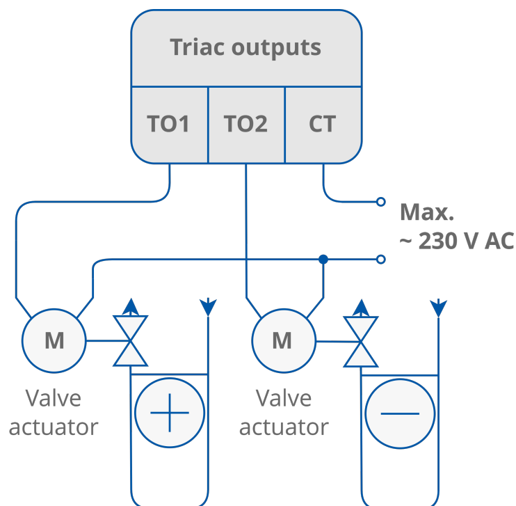
Figure 4. Triac outputs connection
