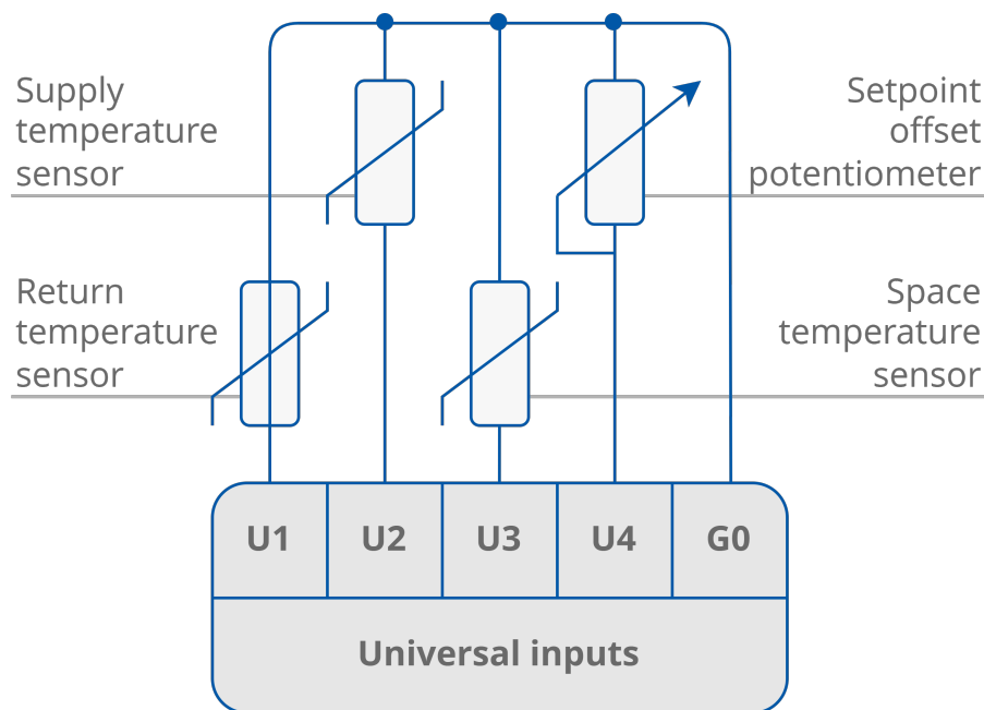
Figure 2. Universal inputs connection
