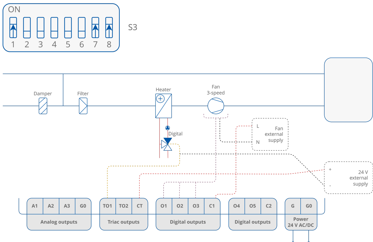
Figure 52. 2-pipe installation with 1-stage digital controlled heating and 3-speed fan
