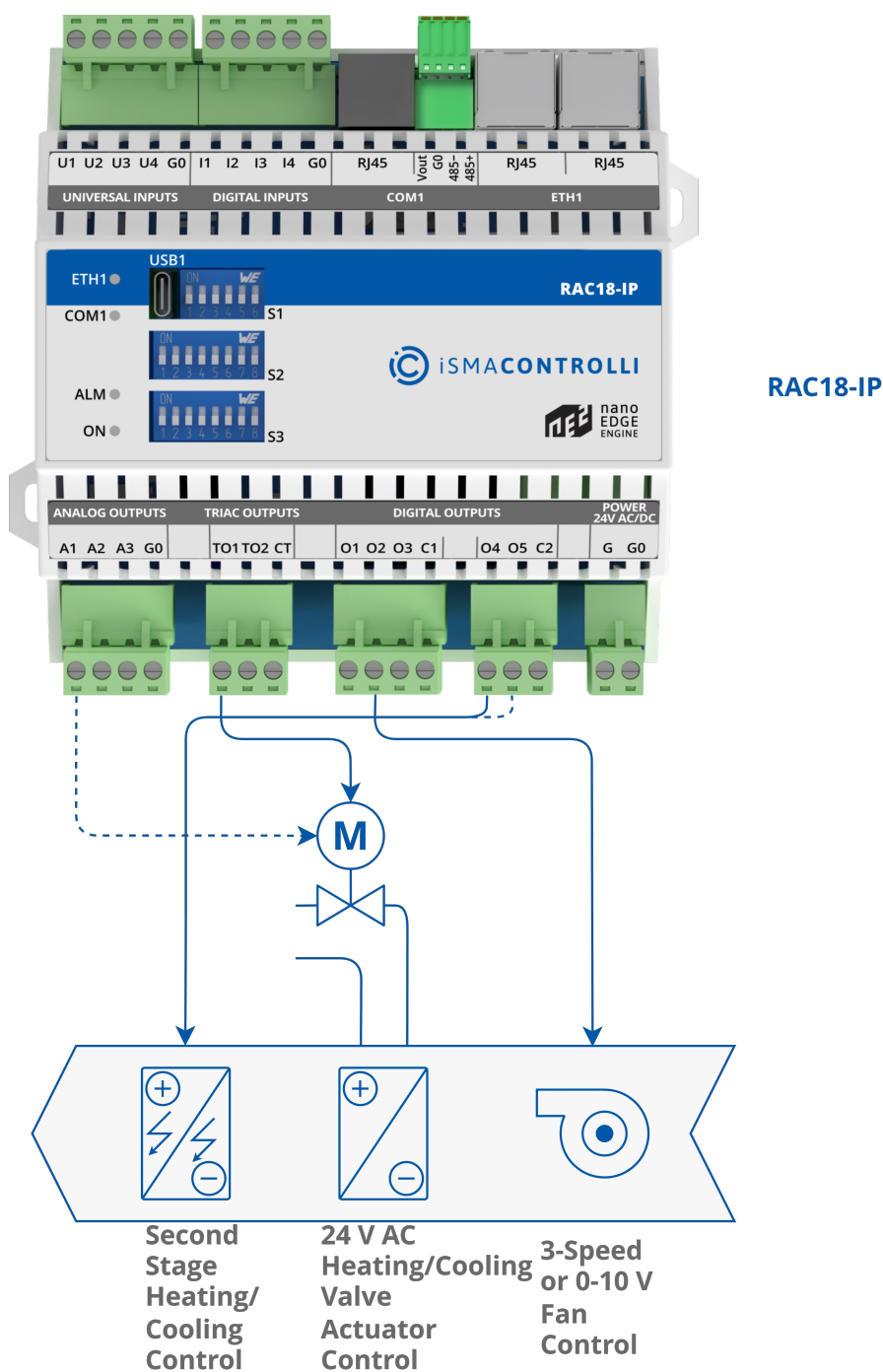
Figure 14. 2-pipe FCU installation
