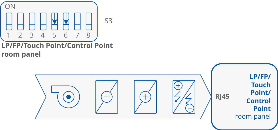
Figure 20. LP/FP/Touch Point/Control Point room panel set as a temperature source
