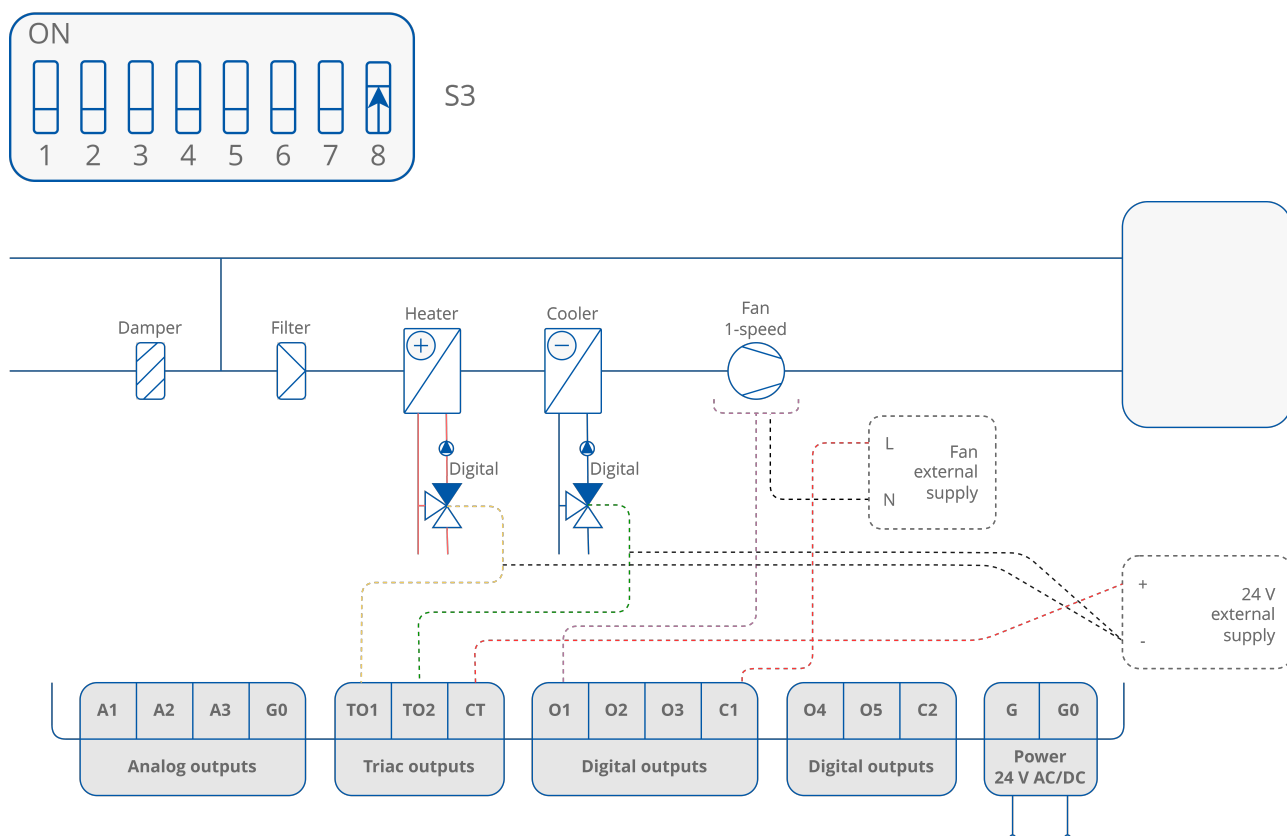
Figure 38. 4-pipe installation with 1-stage digital controlled heating and cooling and 1-speed fan
