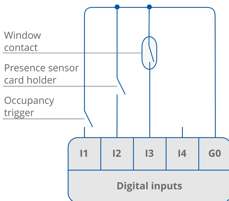
Figure 3. Digital inputs connection
