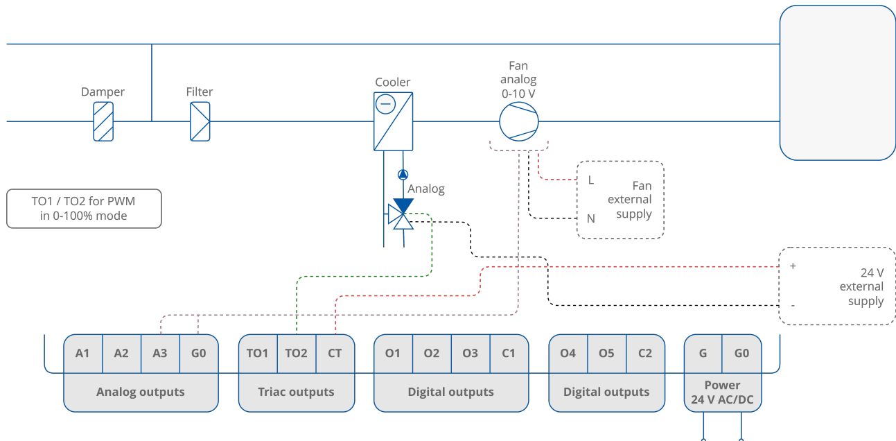
Figure 54. 2-pipe installation with 1-stage analog controlled cooling and analog controlled fan - valve in PWM mode
