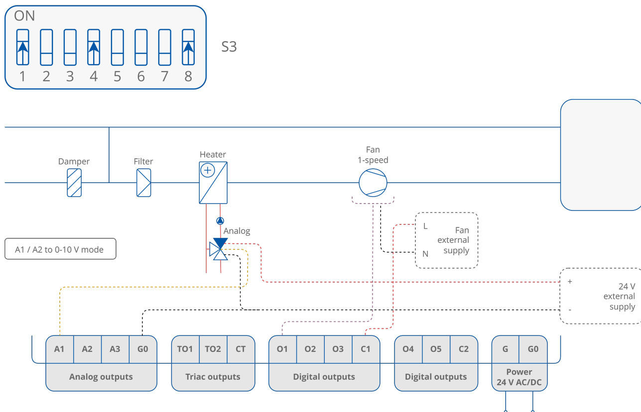
Figure 55. 2-pipe installation with 1-stage analog controlled heating and 1-speed fan - valve in analog mode
