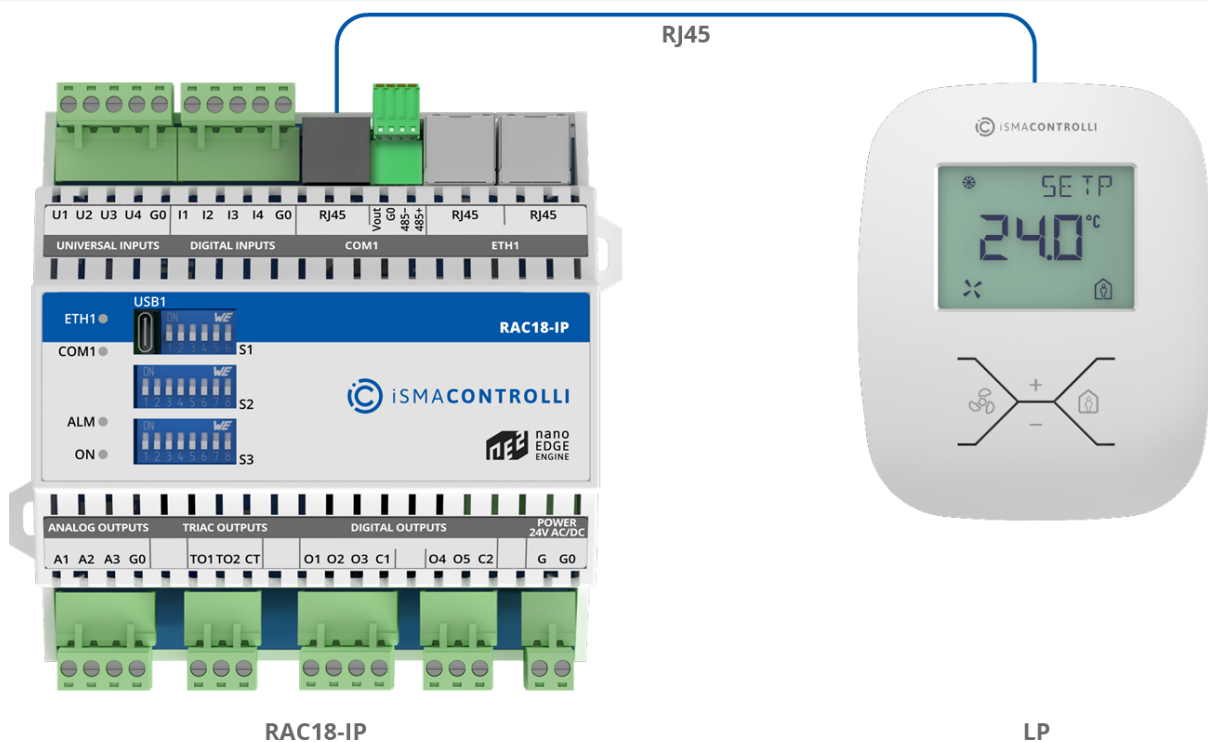
Figure 33. RAC18-IP connection to the LP pane
