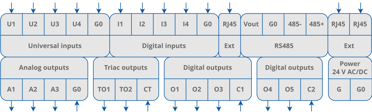
Figure 36. Inputs and outputs overview
