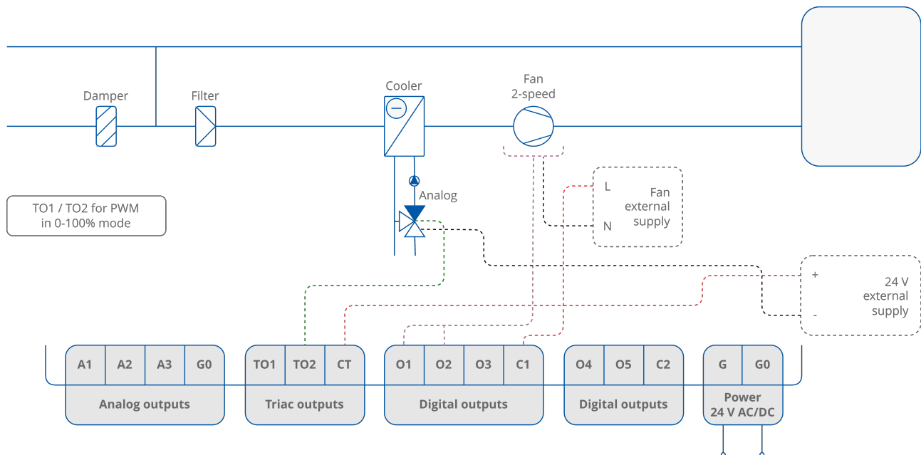
Figure 58. 2-pipe installation with 1-stage analog controlled cooling and 2-speed fan - valve in PWM mode
