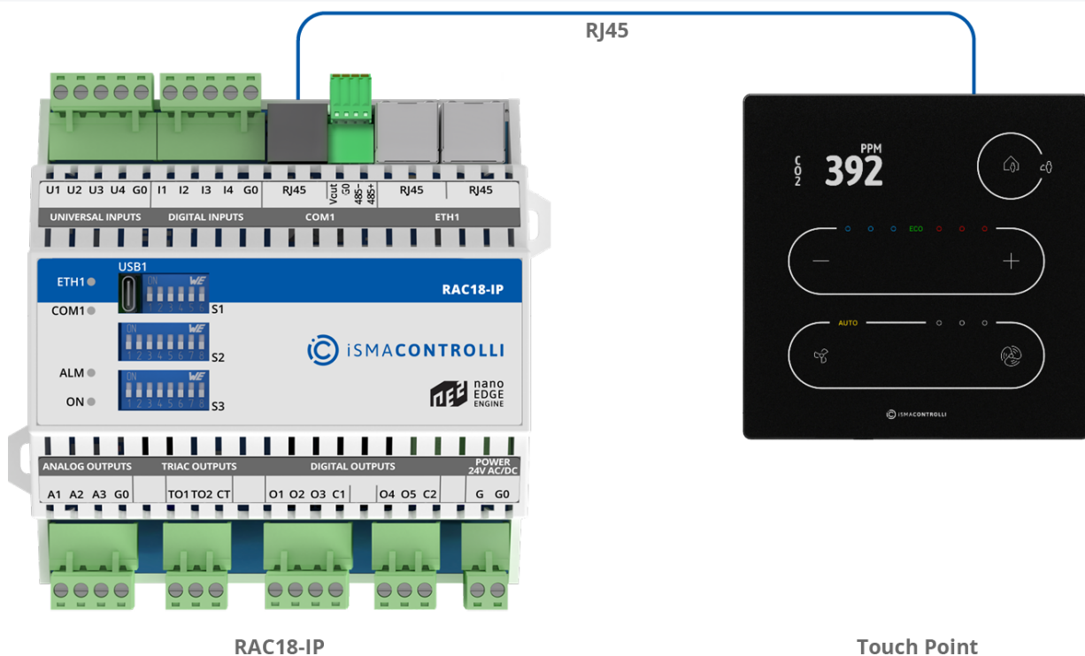
Figure 31. RAC18-IP connection to Touch Point panel
