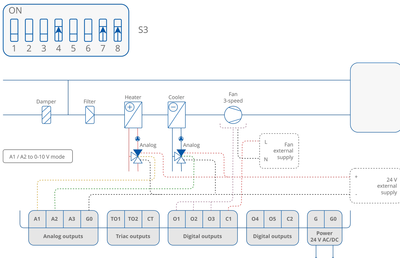
Figure 47. 4-pipe installation with 1-stage analog controlled heating and cooling and 3-speed fan - valve in analog mode
