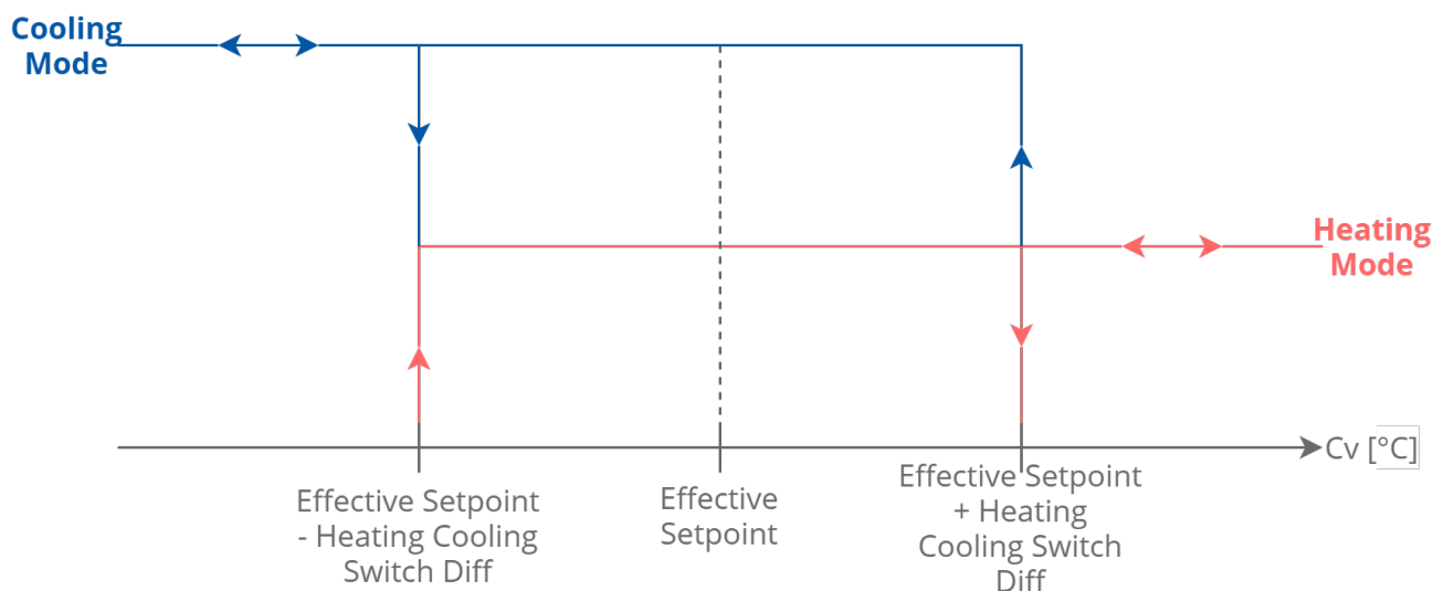
Figure 30. Switching between heating/cooling chart
