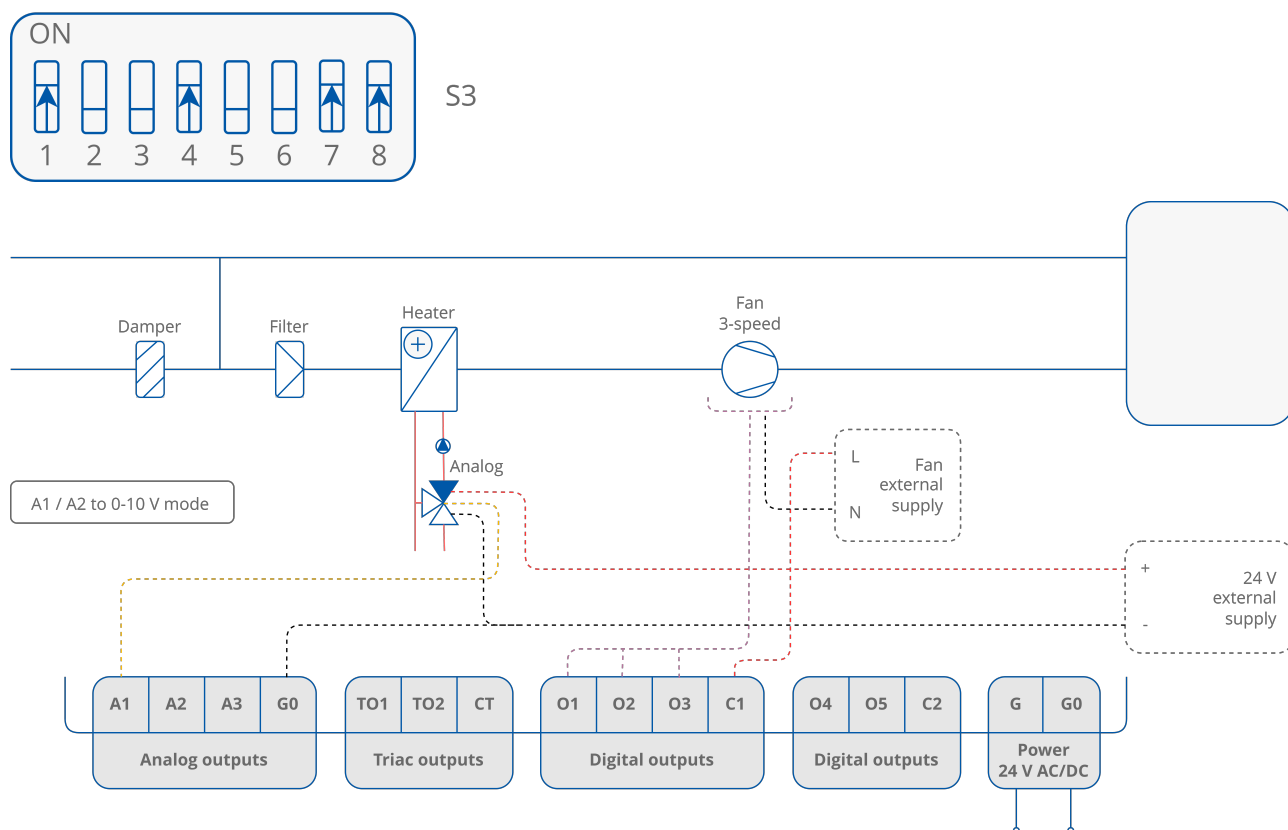
Figure 59. 2-pipe installation with 1-stage analog controlled heating and 3-speed fan - valve in analog mode
