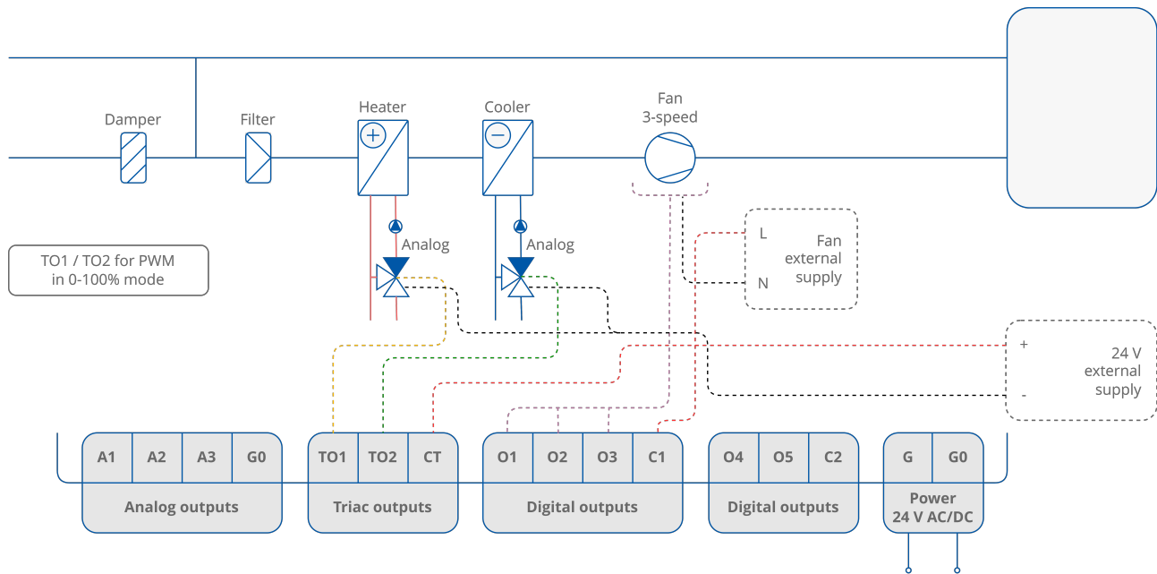
Figure 48. 4-pipe installation with 1-stage analog controlled heating and cooling and 3-speed fan - valve in PWM mode
