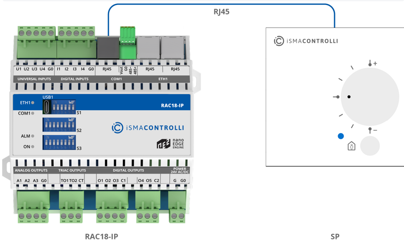
Figure 34. RAC18-IP connection to SP panel
