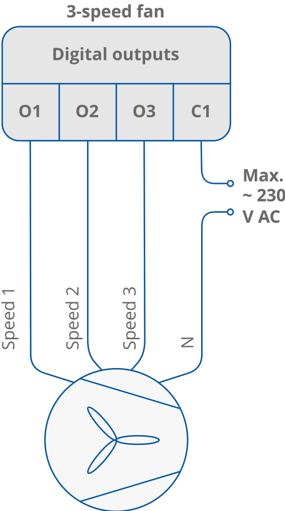
Figure 27. 3-speed fan connection
