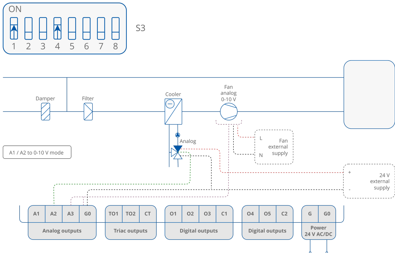
Figure 53. 2-pipe installation with 1-stage analog controlled cooling and analog controlled fan - valve in analog mode
