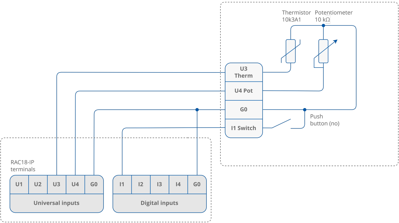
Figure 11. Connection diagram of the iSMA-B-FCU controller
