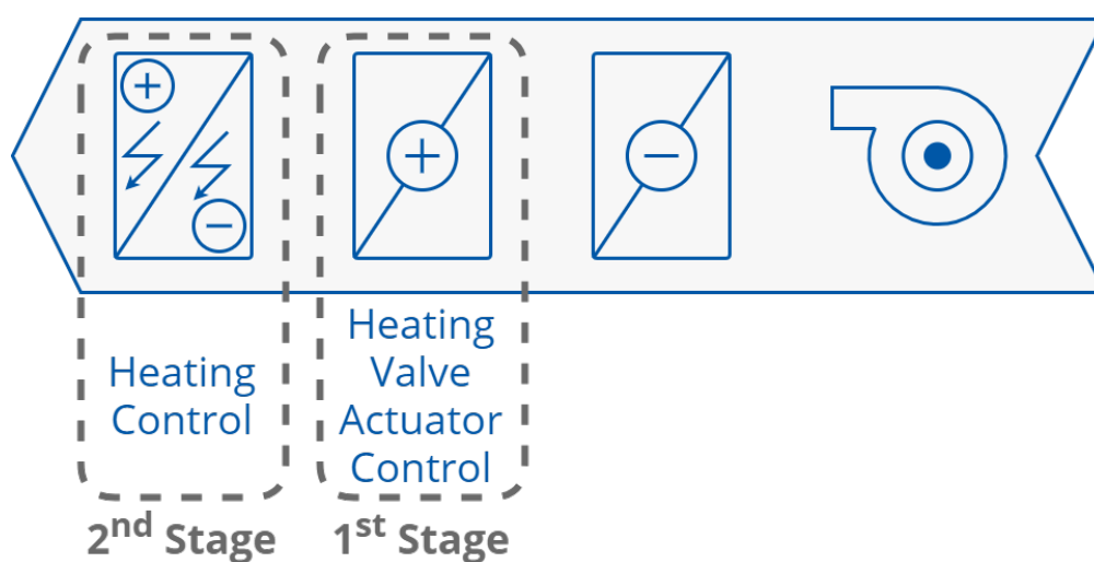
Figure 15. 2 stages of heating in 4-pipe FCU installation
