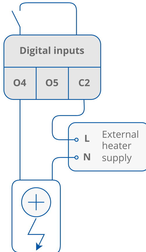
Figure 6. Electrical heater connections
