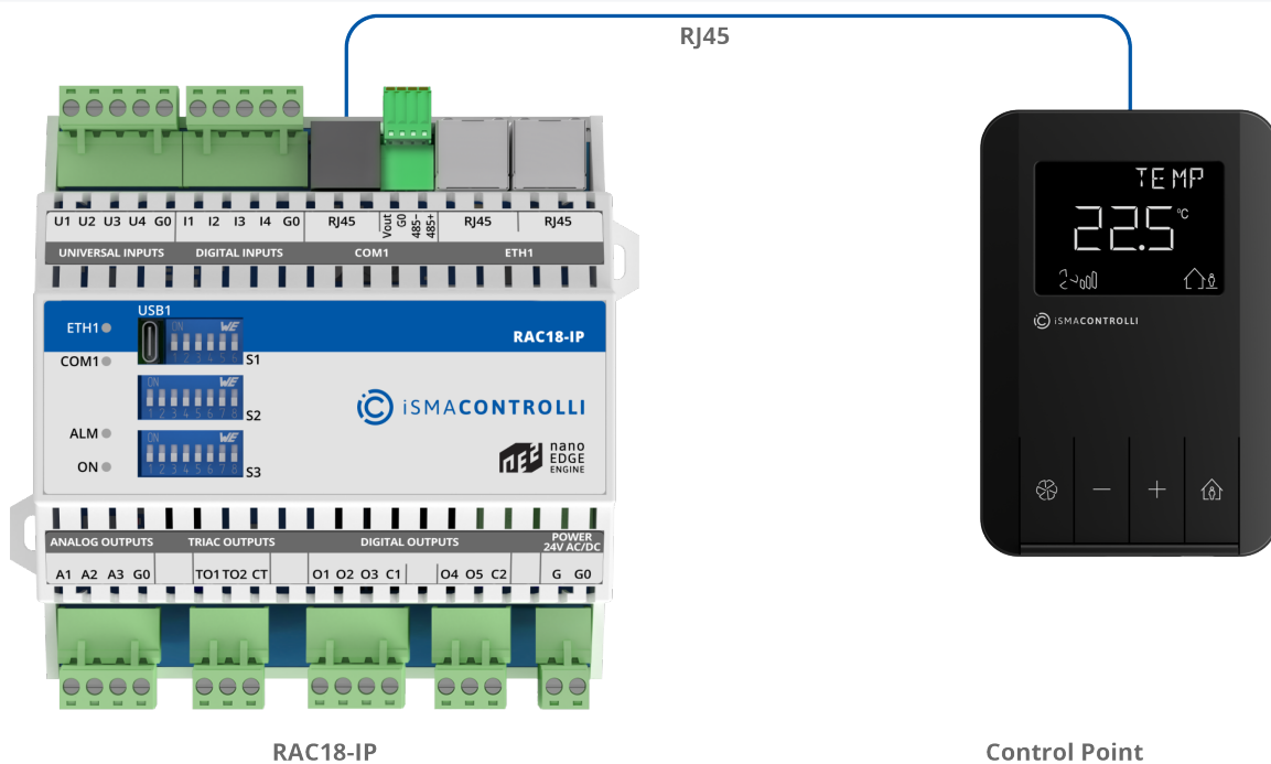
Figure 32. RAC18-IP connection to Control Point panel
