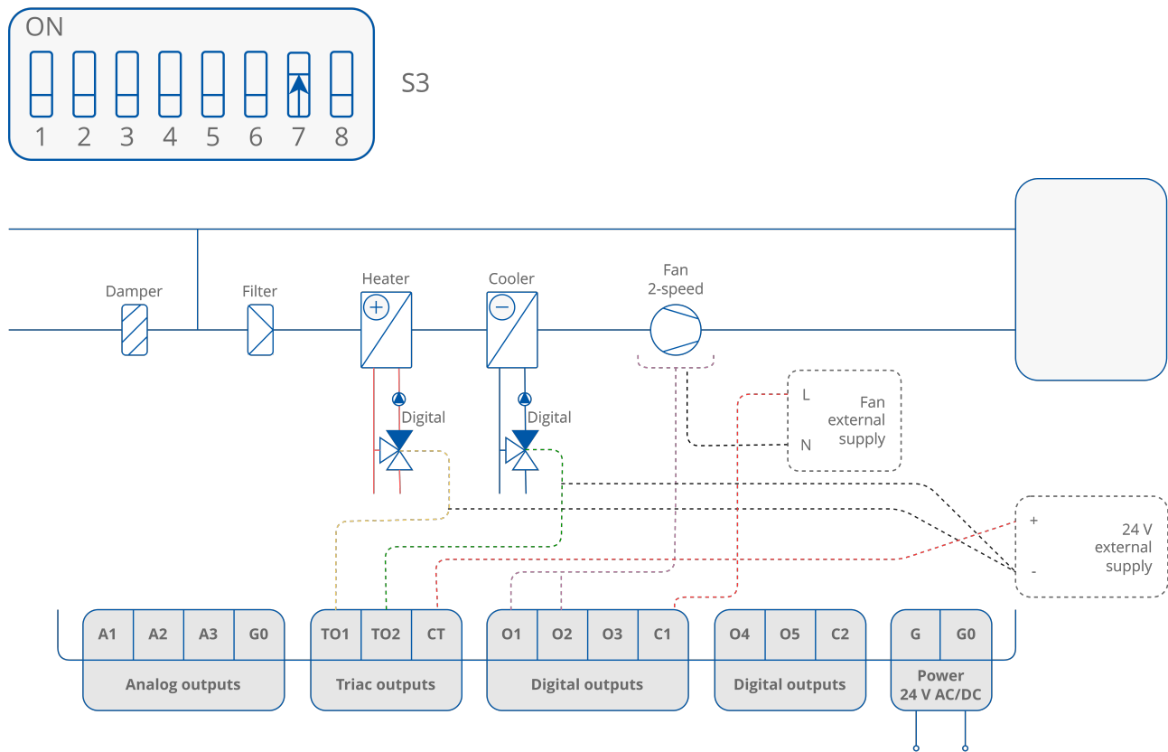
Figure 39. 4-pipe installation with 1-stage digital controlled heating and cooling and 2-speed fan
