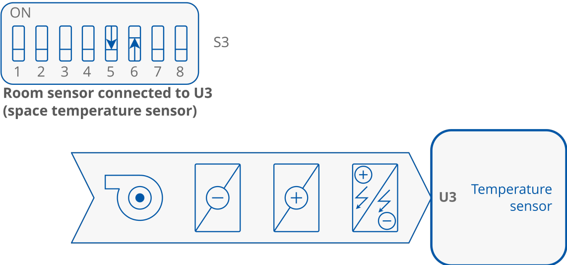
Figure 21. Temperature sensor connected to S3 as a temperature control value source
