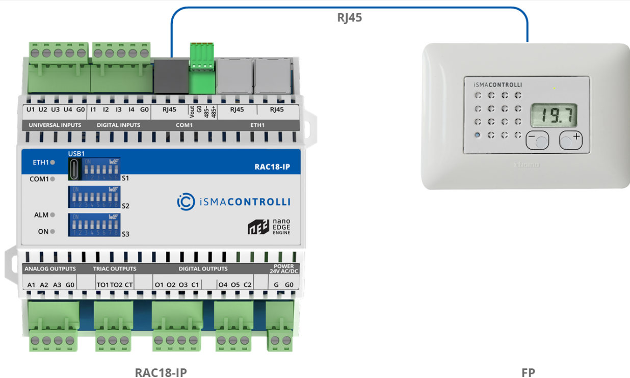
Figure 35. RAC18-IP connection to FP panel
