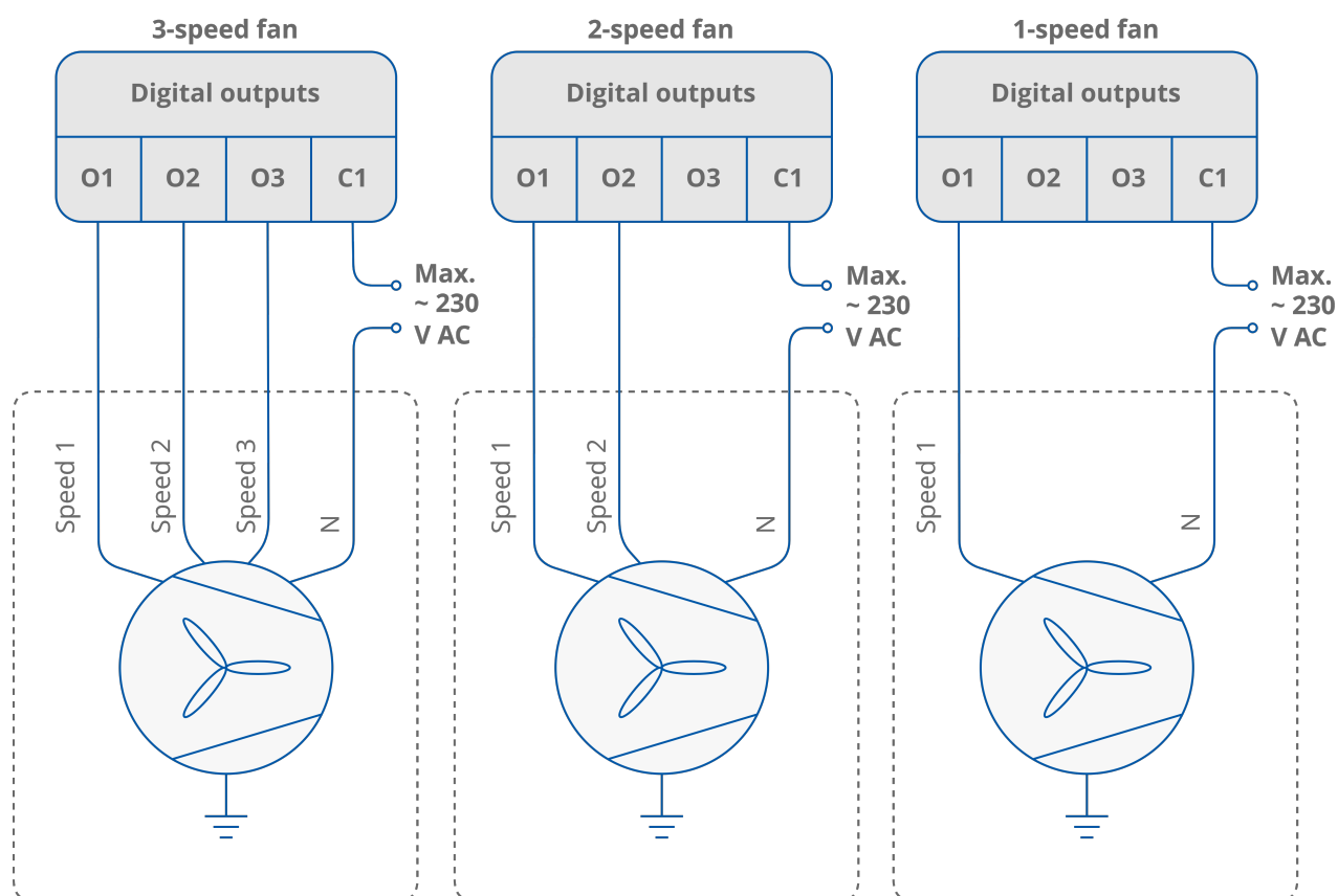
Figure 5. Fan connections
