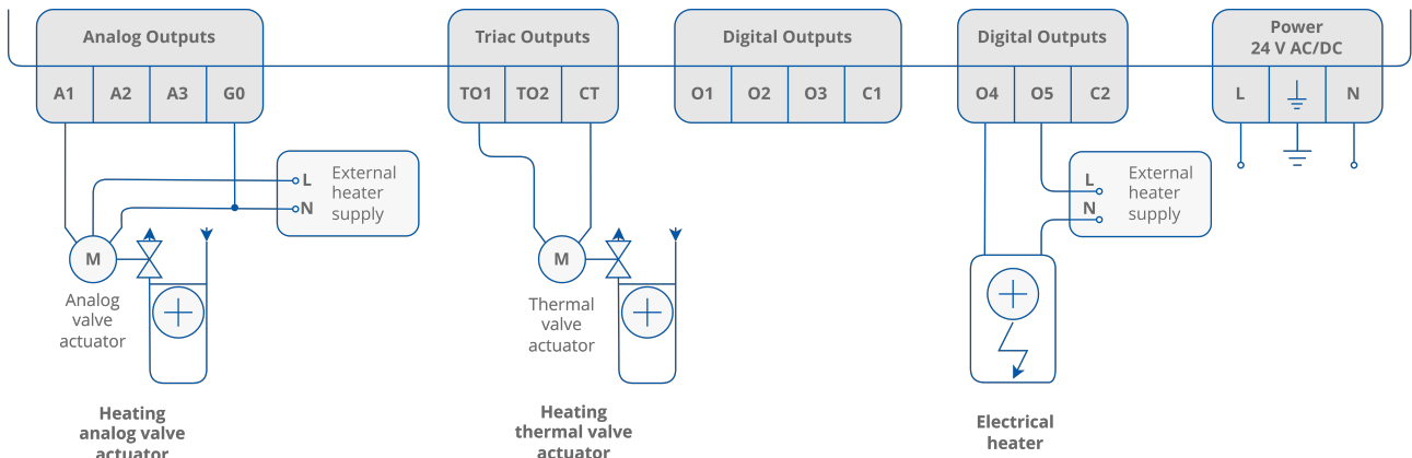
Figure 17. Heating actuators connection
