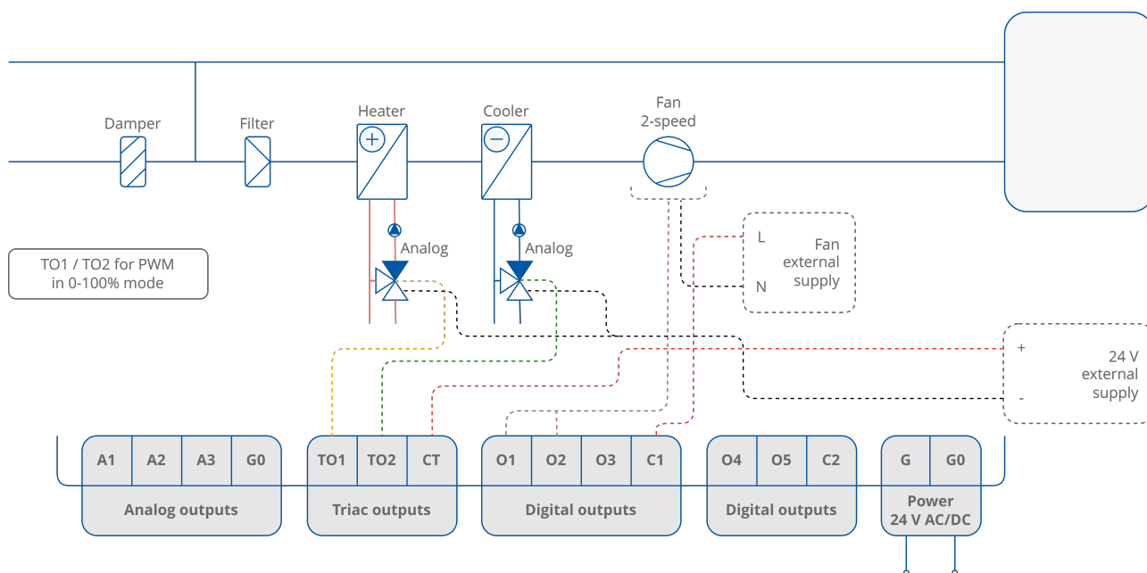
Figure 46. 4-pipe installation with 1-stage analog controlled heating and cooling and 2-speed fan - valve in PWM mode
