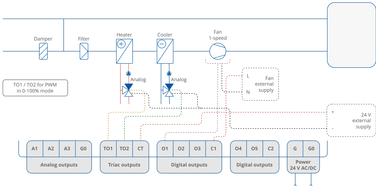
Figure 44. 4-pipe installation with 1-stage analog controlled heating and cooling and 1-speed fan - valve in PWM mode
