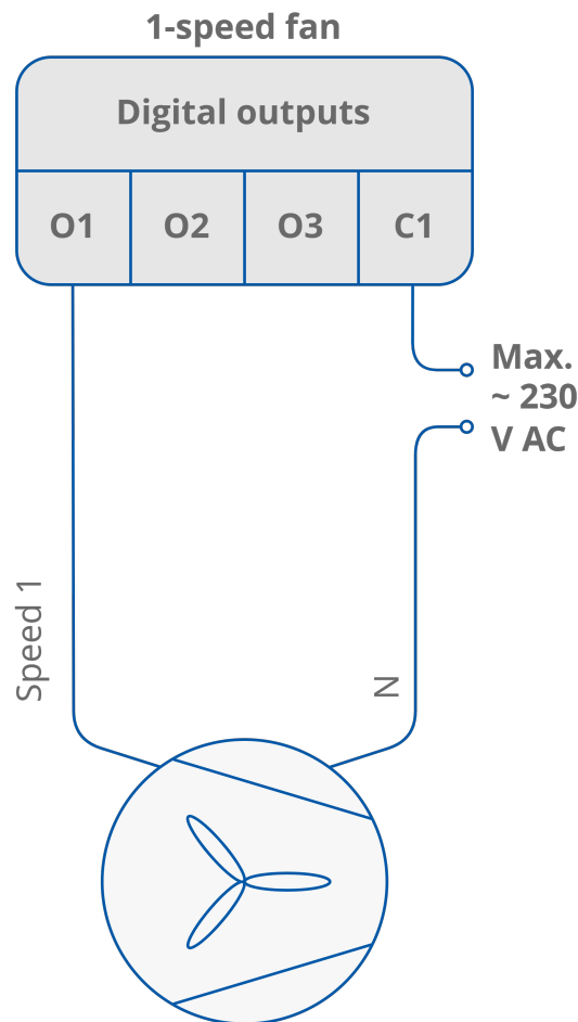
Figure 25. 1-speed fan connection
