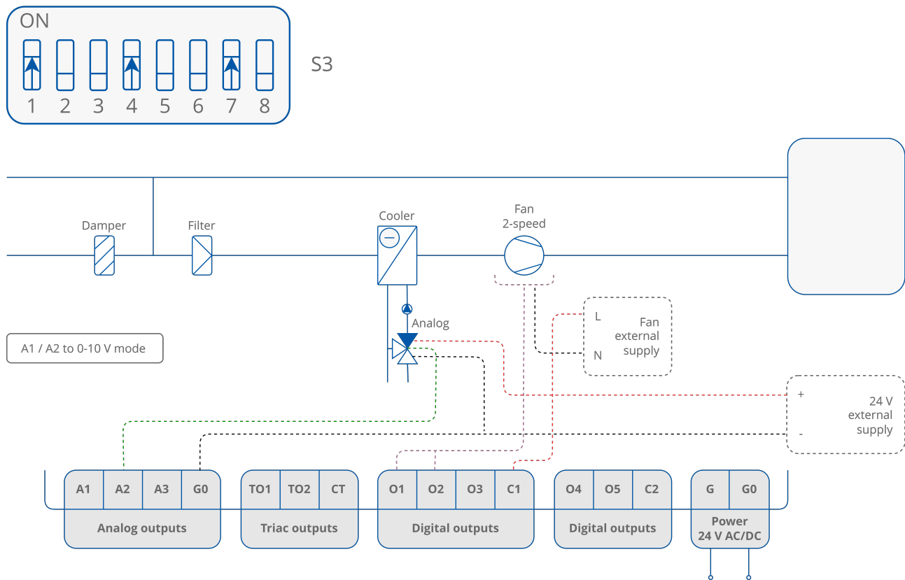
Figure 57. 2-pipe installation with 1-stage analog controlled cooling and 2-speed fan - valve in analog mode
