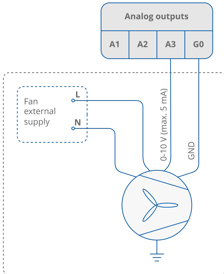
Figure 9. Connection of analog fan control
