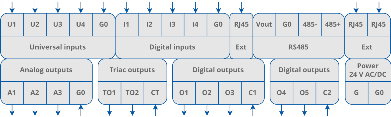
Figure 19. RAC18-IP connectors
