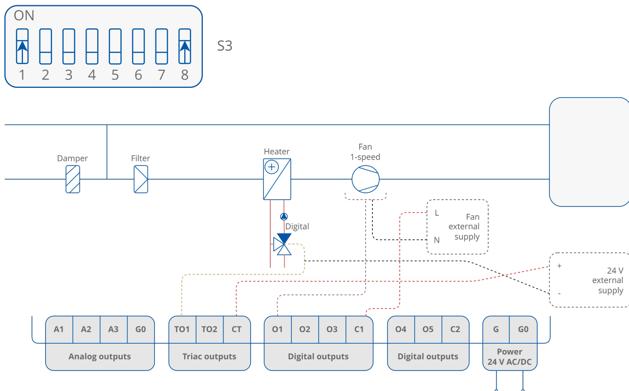
Figure 50. 2-pipe installation with 1-stage digital controlled heating and 1-speed fan
