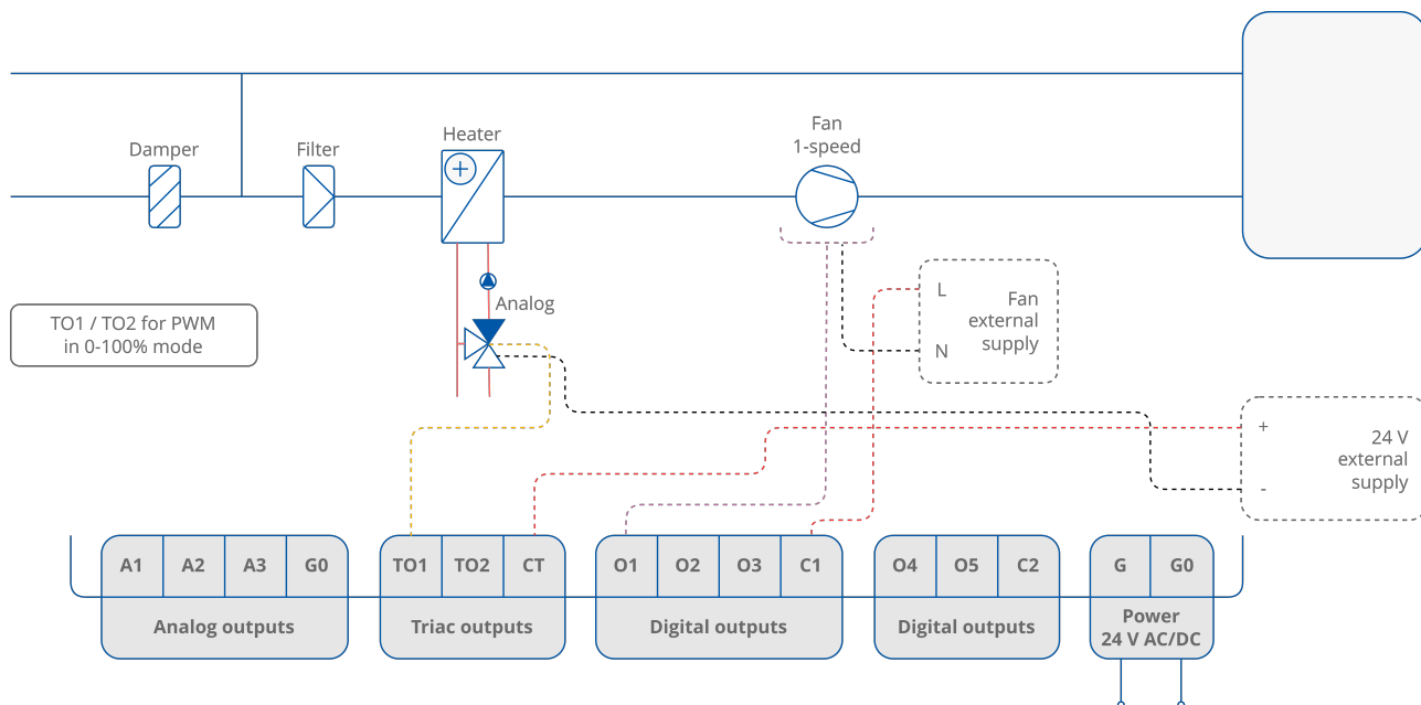
Figure 56. 2-pipe installation with 1-stage analog controlled heating and 1-speed fan - valve in PWM mode
