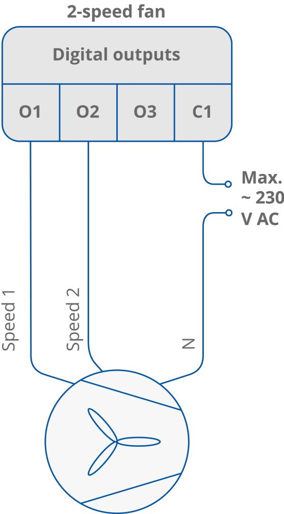
Figure 26. 2-speed fan connection
