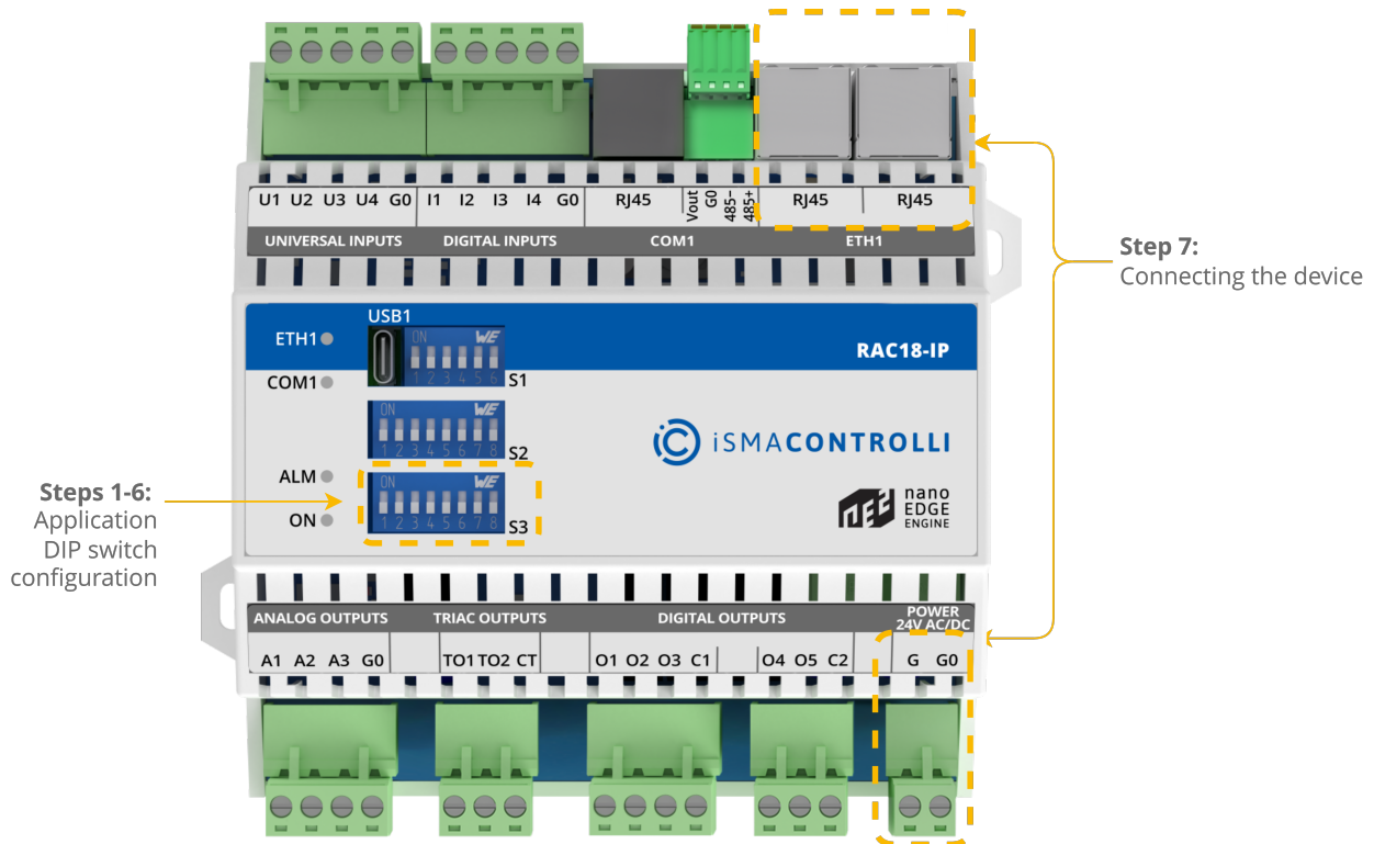
Figure 12. RAC18-IP controller
