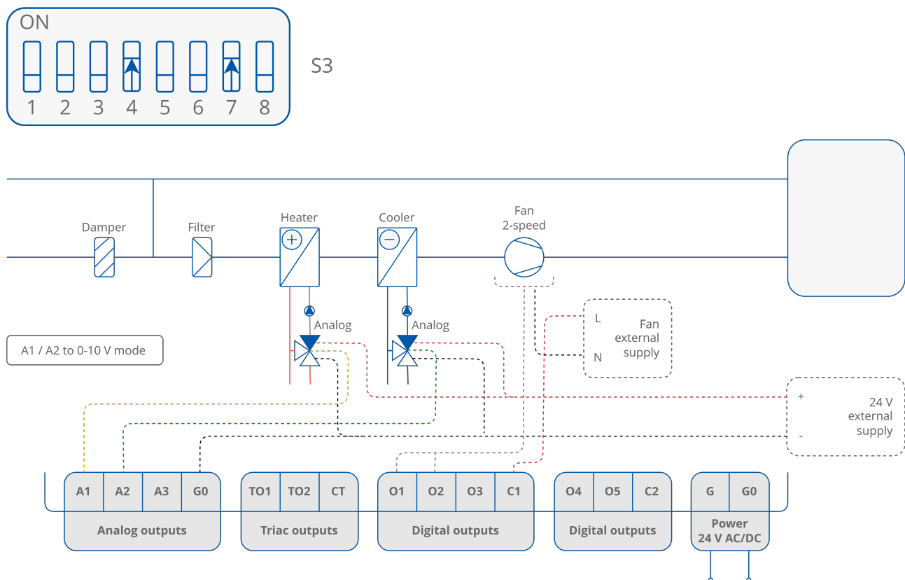
Figure 45. 4-pipe installation with 1-stage analog controlled heating and cooling and 2-speed fan - valve in analog mode
