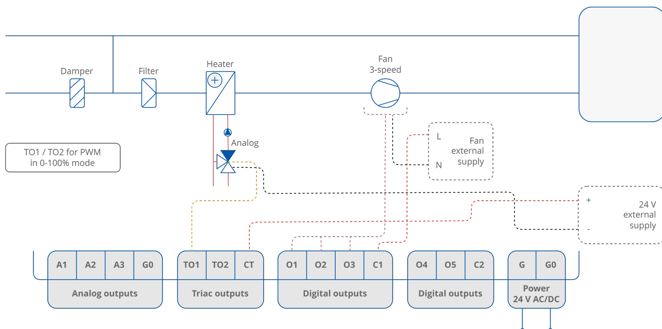
Figure 60. 2-pipe installation with 1-stage analog controlled heating and 3-speed fan - valve in PWM mode
