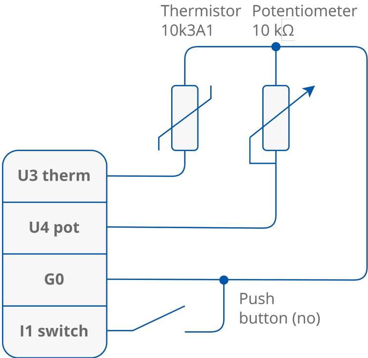
Figure 10. Diagram of internal connections of the simple panel
