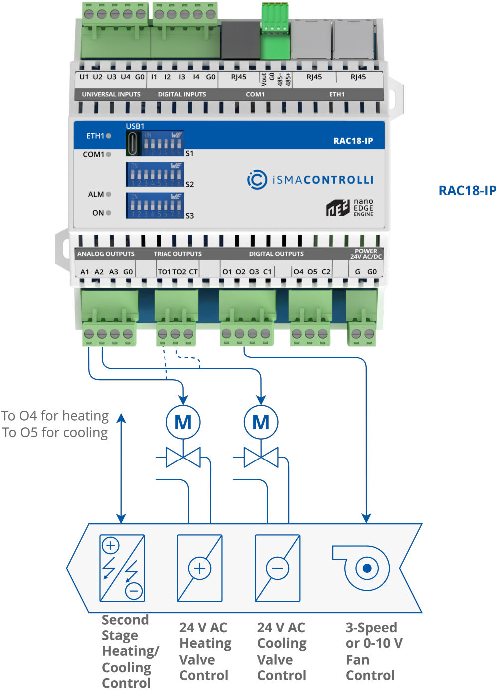
Figure 13. RAC18-IP controller
