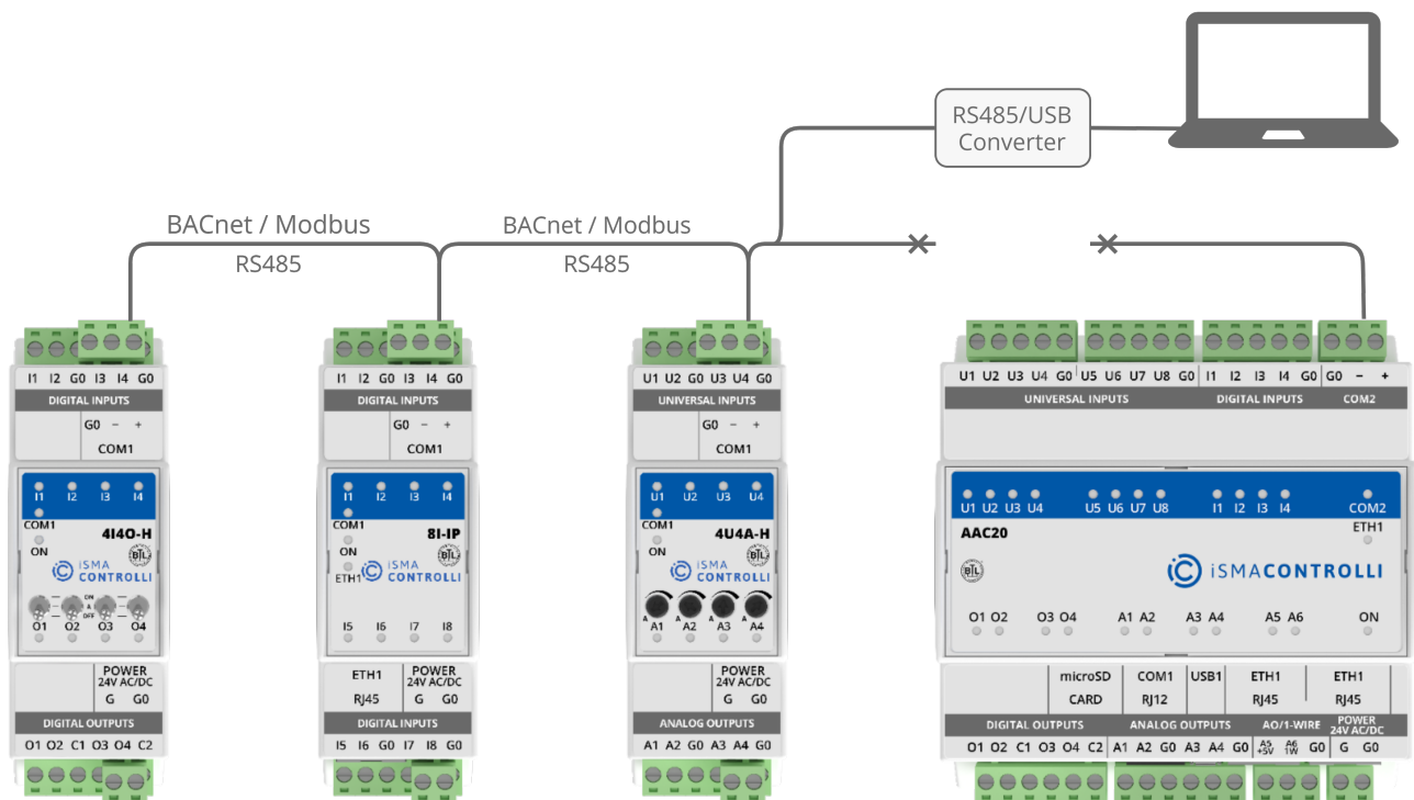
Figure 4. RS485 converter
