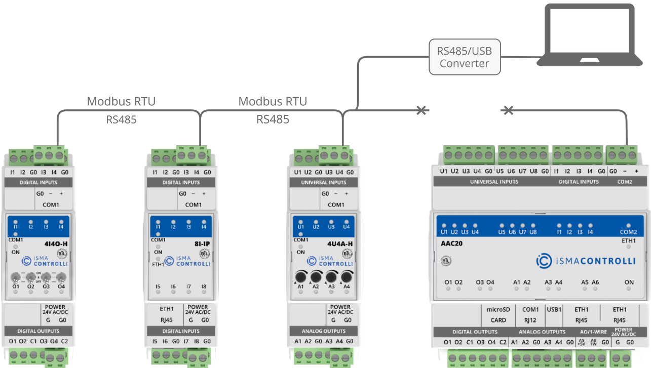
Figure 31. Devices connected directly via Modbus RS485
