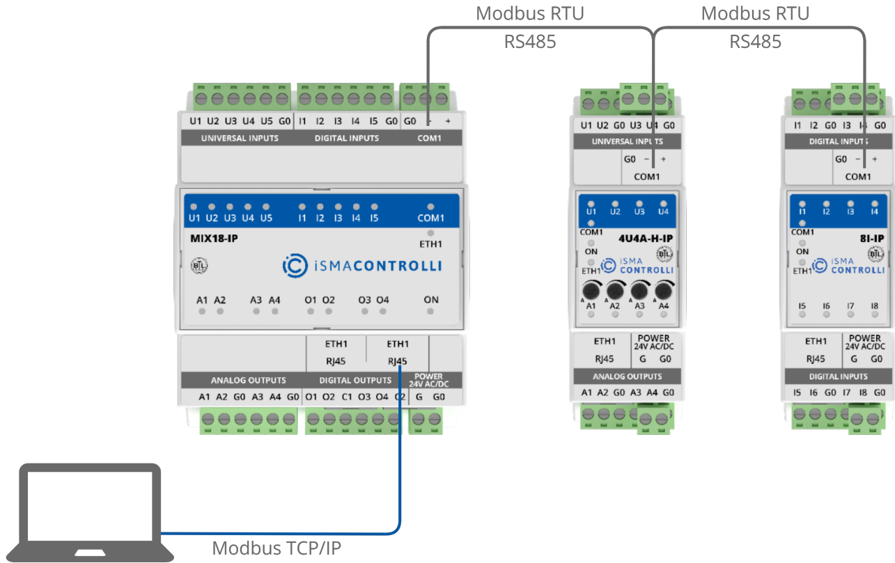
Figure 25. Devices connected to IP gateway via RS485
