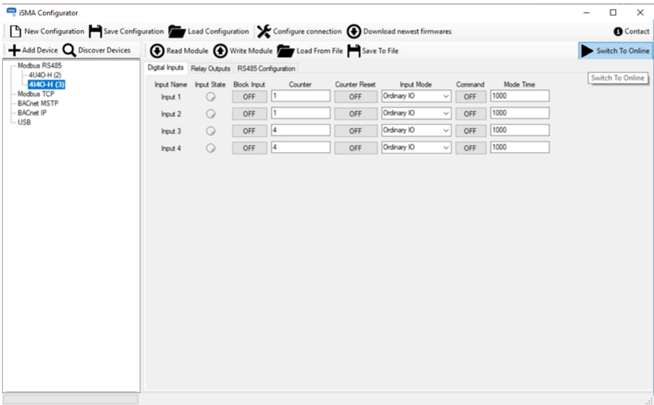
Figure 34. Device discovered via Modbus RS485
