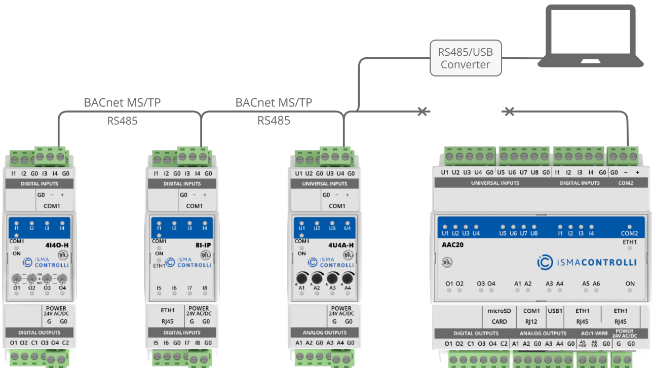
Figure 30. Devices connected via BACnet MS/TP
