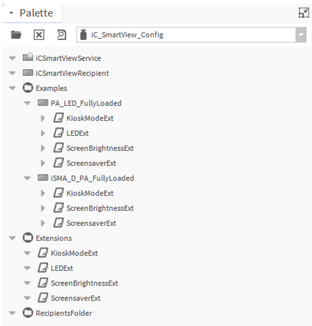
Figure 5. All contents of the iC SmartView Config palette
