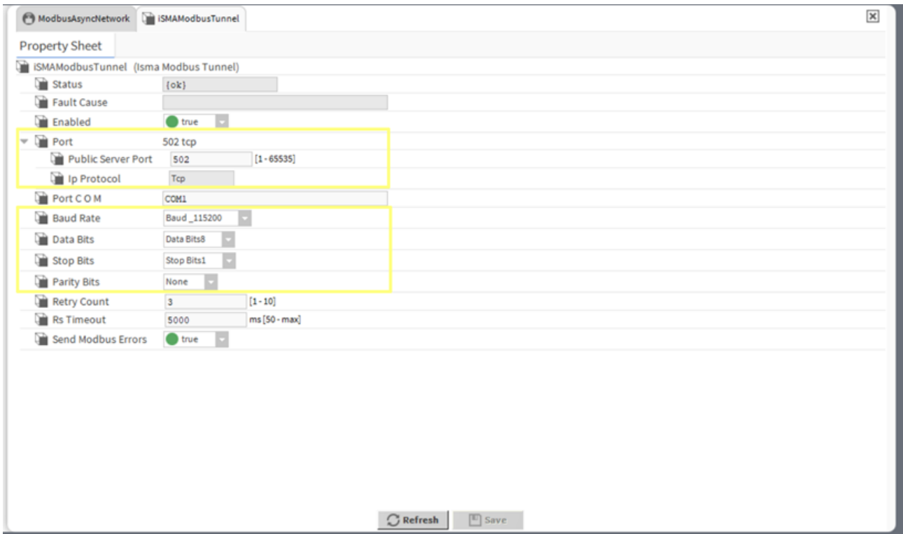
Figure 33. Communication parameters for the iSMA Modbus Tunnel
