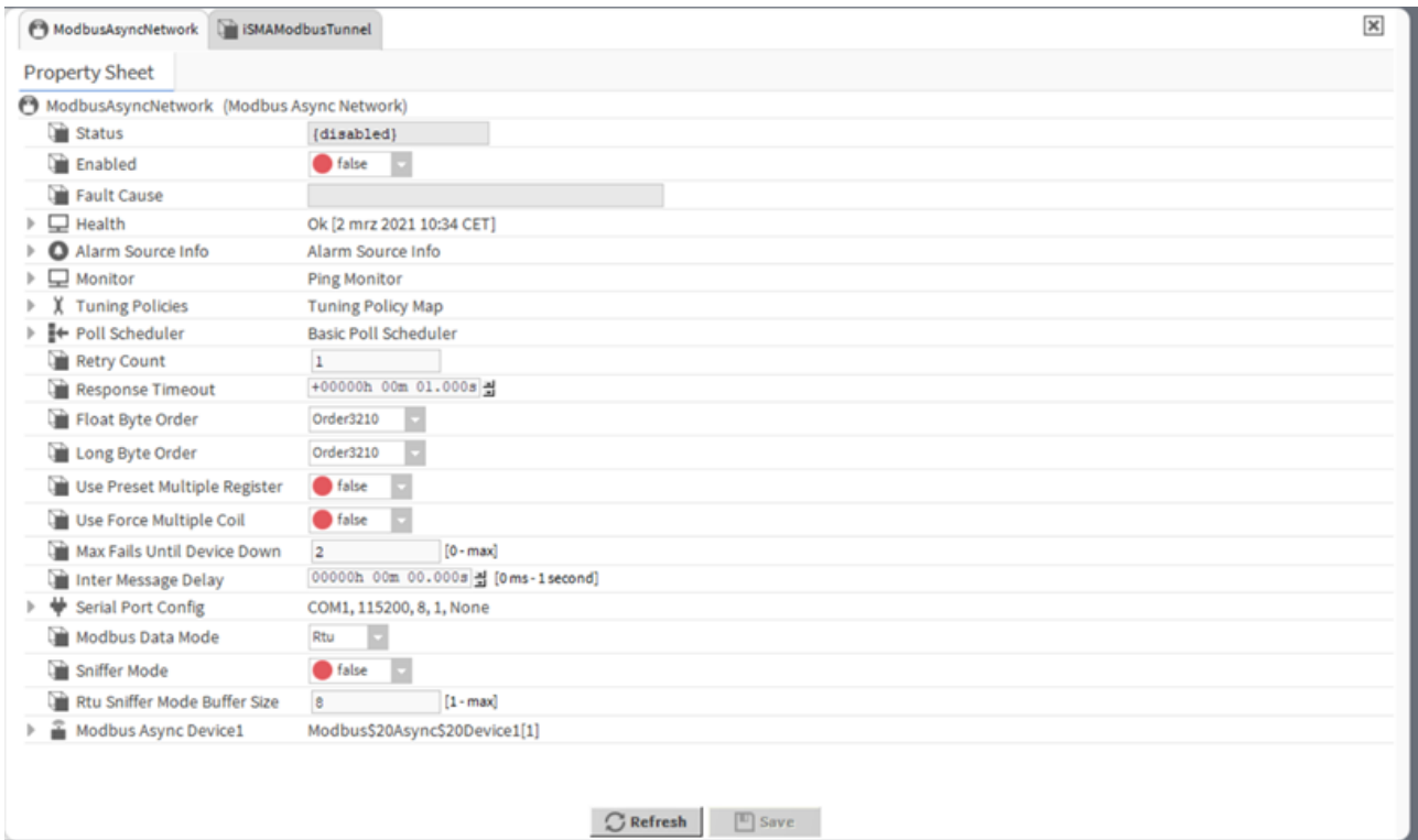
Figure 32. ModbusAsyncNetwork disabled on the iSMA-B-MAC39NL controller
