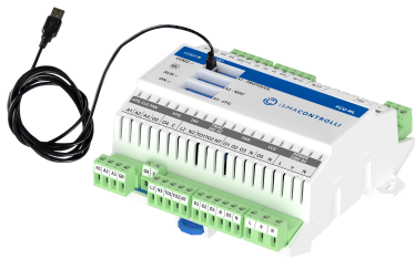
Figure 49. FCU controller panel USB connection
