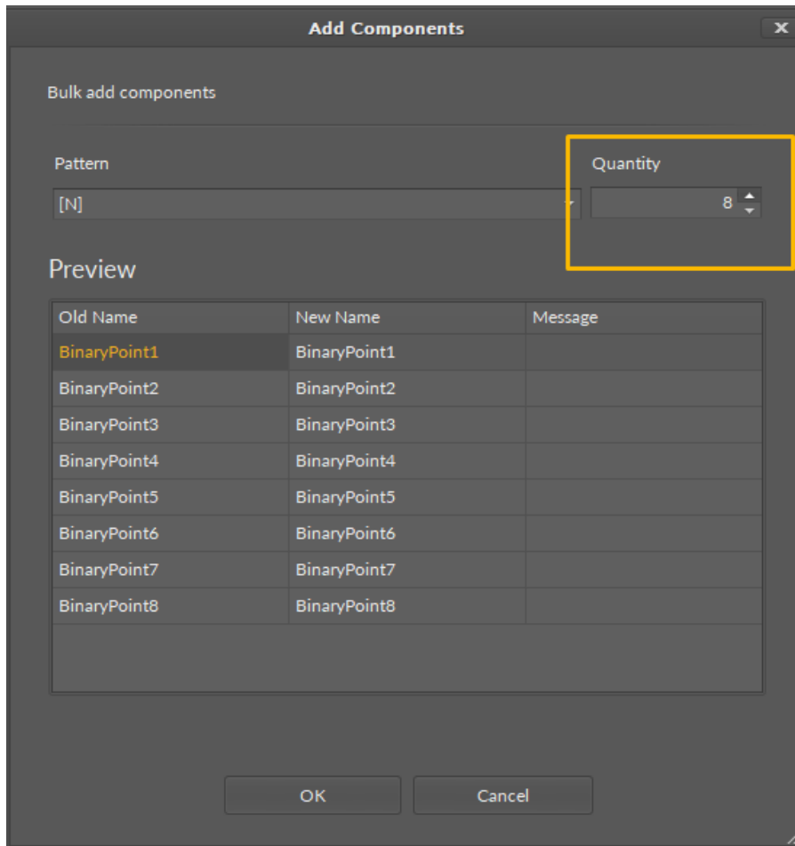
Figure 41. Dialog window
