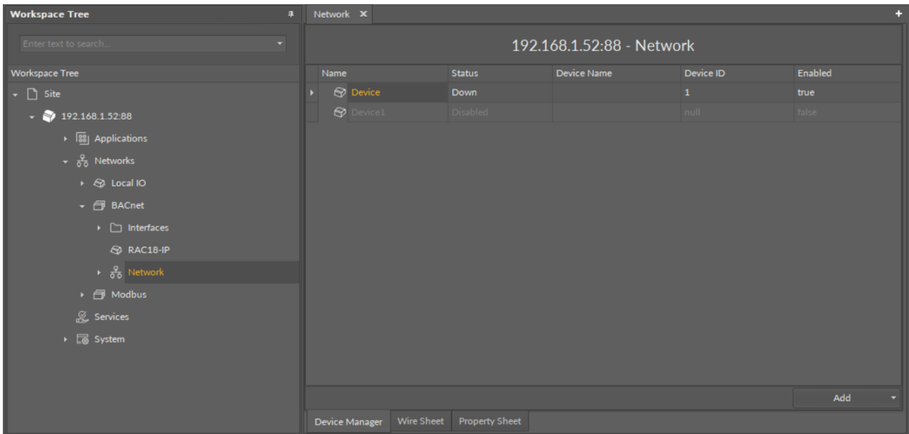
Figure 50. Device Manager
