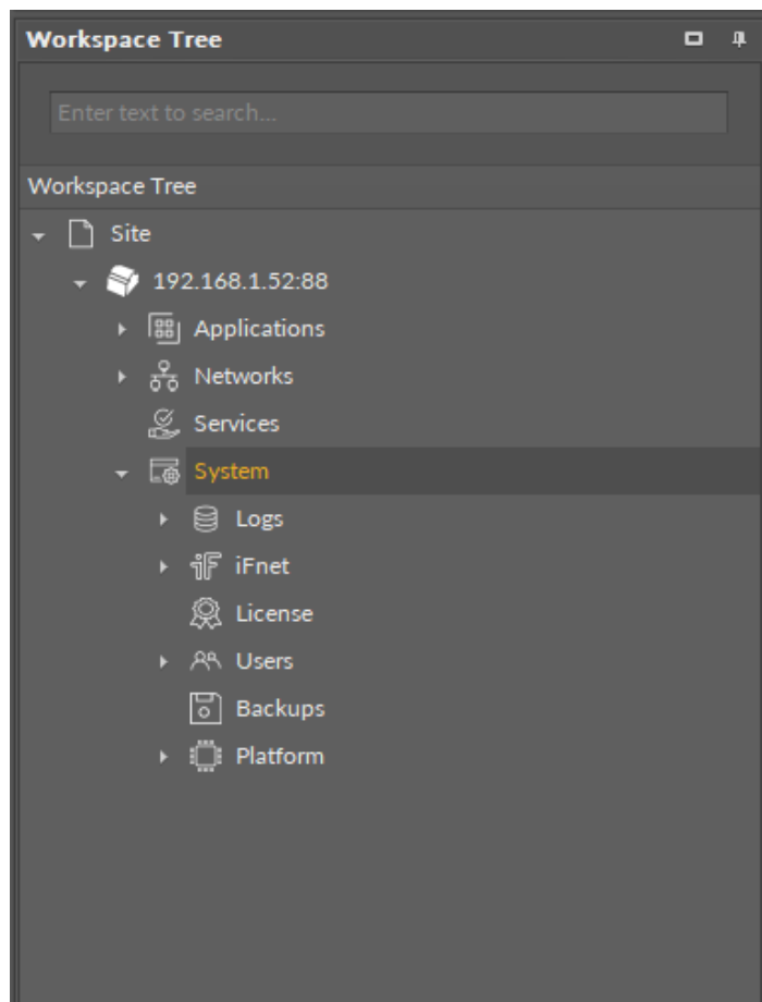
Figure 59. System container
