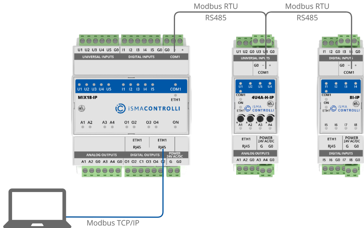
Figure 24. Devices connected to IP gateway via RS485
