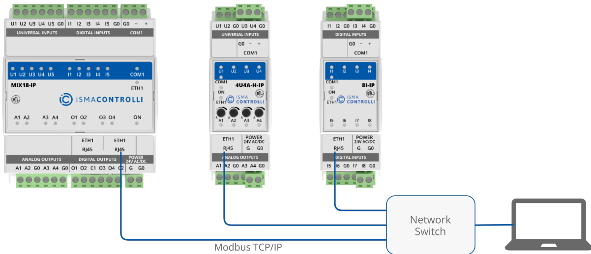
Figure 22. Device connected via Modbus TCP/IP
