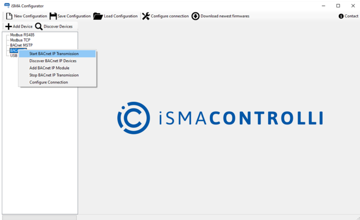
Figure 33. Starting BACnet IP transmission
