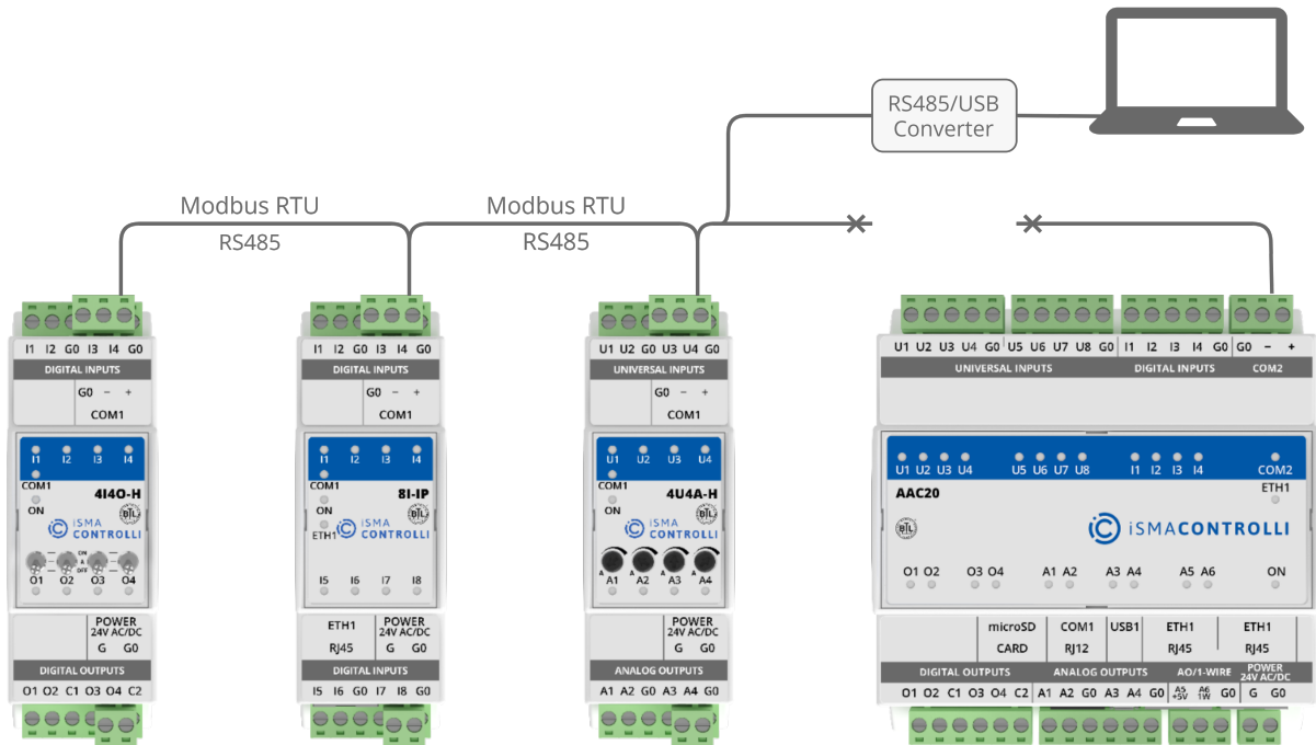
Figure 18. Devices connected directly via Modbus RS485
