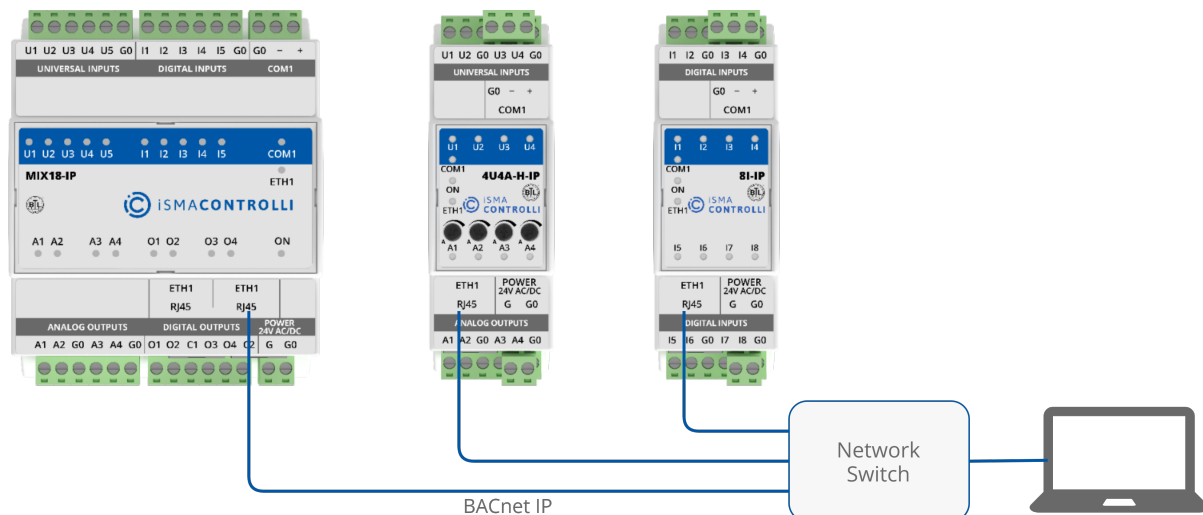
Figure 30. Devices connected via BACnet IP
