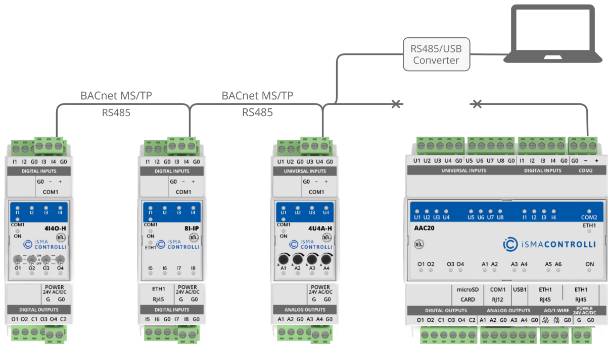
Figure 29. Devices connected via BACnet MS/TP
