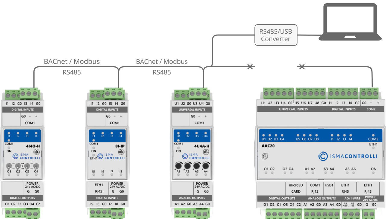
Figure 4. An RS485 converter
