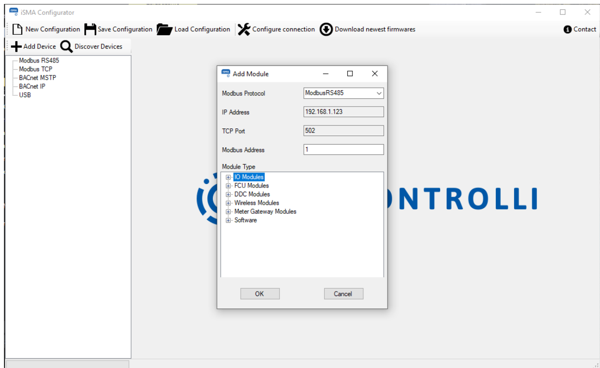
Figure 36. Adding Modbus device manually
