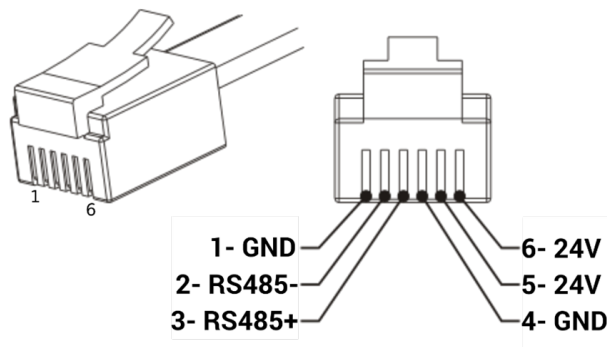
Figure 5. RJ12 pins
