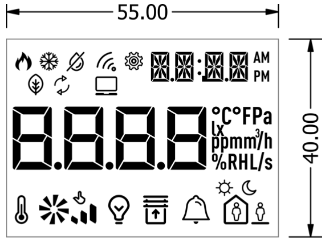
Figure 14. The ICD display general view
