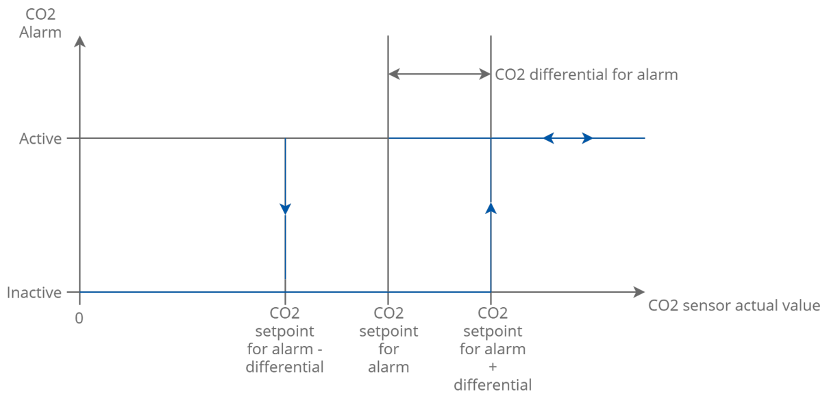
Figure 17. CO2 alarm with differential for active alarm
