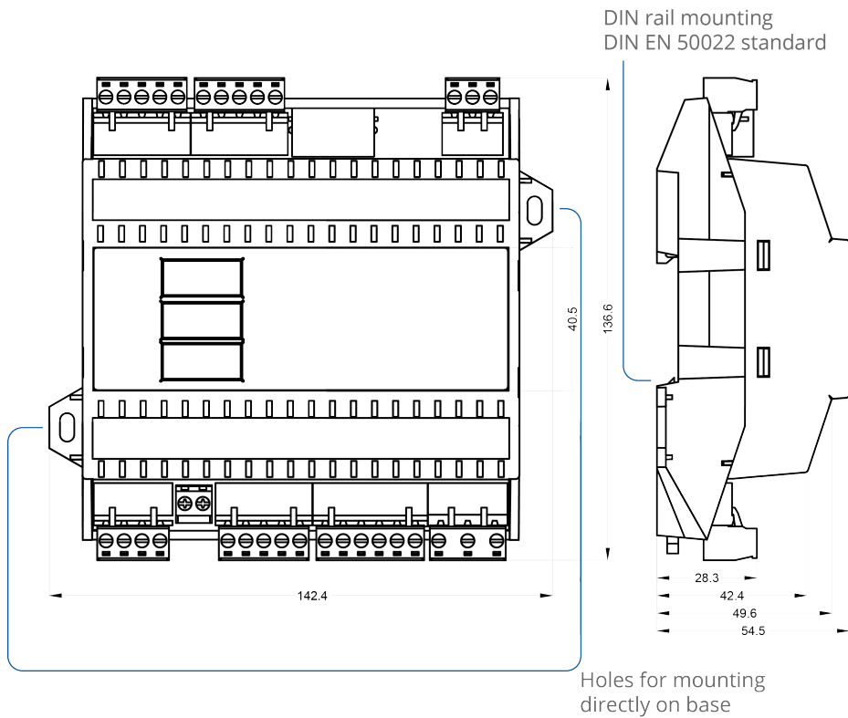
Figure 1. FCU dimensions and mounting
