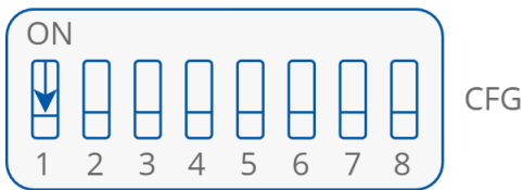
4-pipe-heating and cooling
